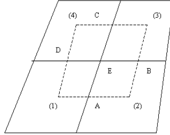
Figure 3: A cluster with its interaction region for computing the flux across [EA],[EB],[EC] and [ED] in a quadrilateral grid.
