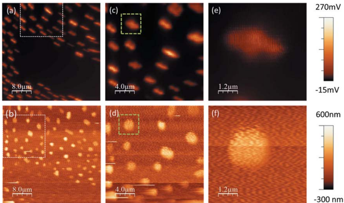
Figure 4 (a, c, e) Scanning X-ray diffraction maps and (b, d, f) simultaneously recorded AFM topography images of Au islands on sapphire substrate. The dashed squares in (a) and (b) mark the area imaged in (c) and (d) while the dotted squares in the latter images indicate the areas imaged in (e) and (f). All images were recorded at the Au222 Bragg reflection ( \theta = 36.20^\circ ).
