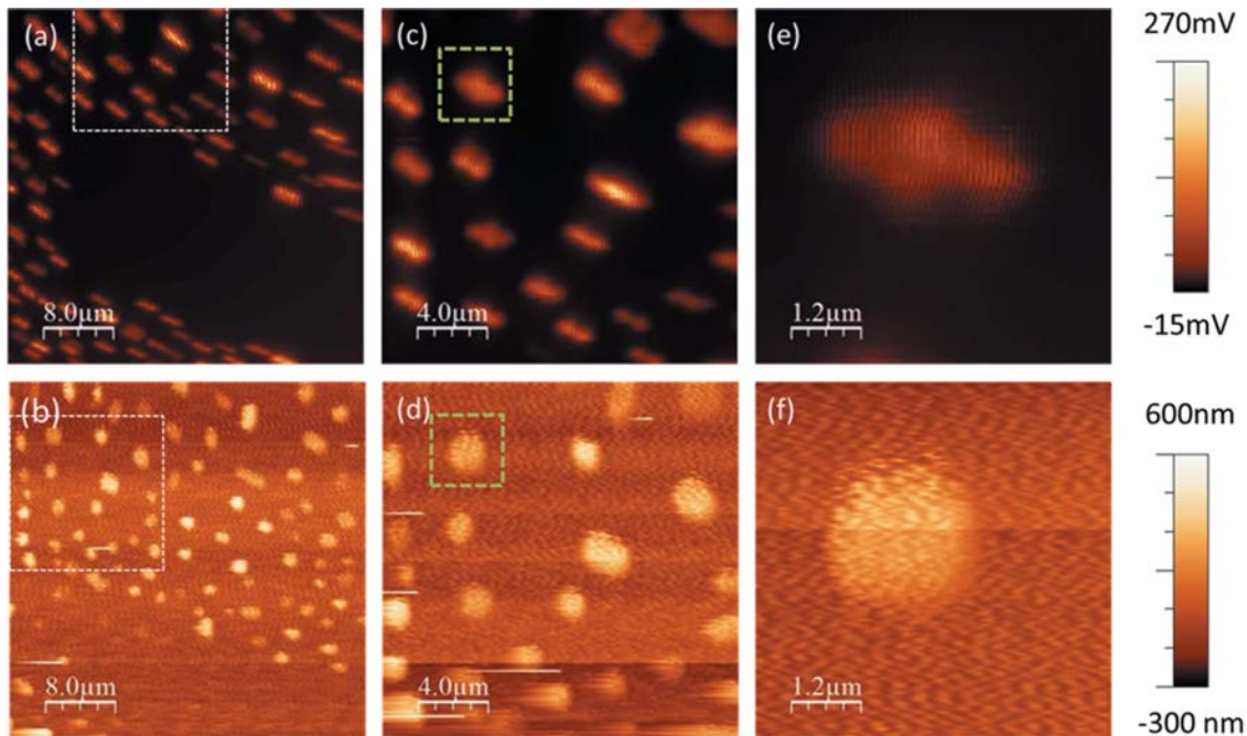
Figure 4 (a, c, e) Scanning X-ray diffraction maps and (b, d, f) simultaneously recorded AFM topography images of Au islands on sapphire substrate. The dashed squares in (a) and (b) mark the area imaged in (c) and (d) while the dotted squares in the latter images indicate the areas imaged in (e) and (f). All images were recorded at the Au222 Bragg reflection ( \theta = 36.20^\circ ).
