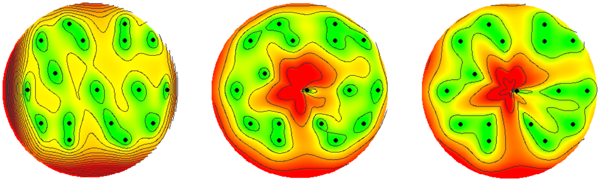
Cartesian GP
