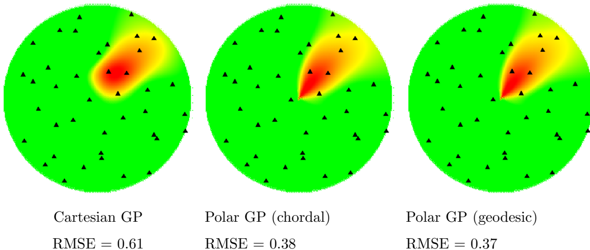
Figure 7: Estimated gas concentrations according to wind speed ( \rho ) and direction ( \theta ), for untrended Cartesian and polar GPs. Adding a Zernike polynomial trend does not improve the results. Triangles correspond to design points.
