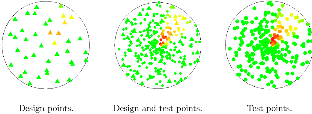
Figure 6: Color representation of gas concentrations. The 242 simulation locations are shown in the middle, including 30 design points (triangles, left) and 212 test points (bullets, right).
