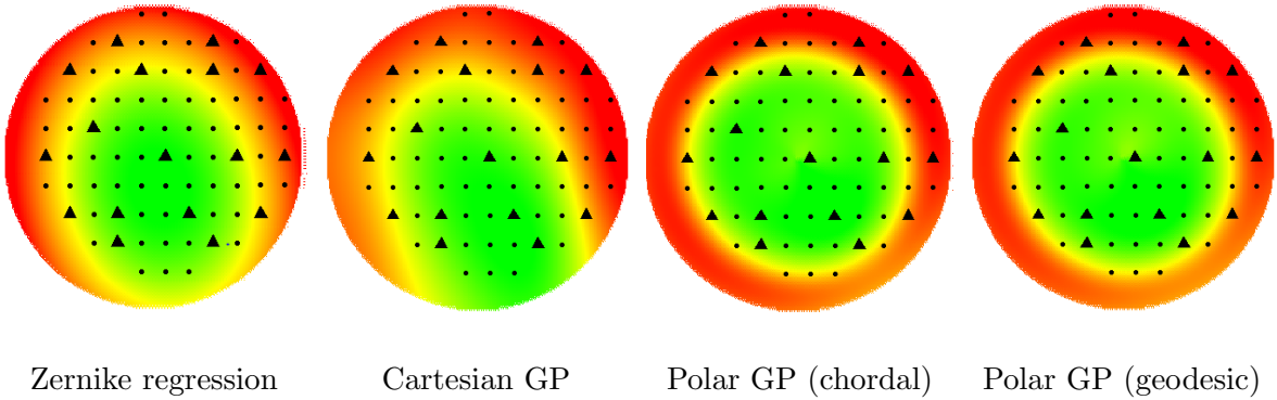
Figure 5: Prediction surface for the best untrended GP models of Table 1. When adding a Zernike trend, the prediction surface is approximately the same as for a pure Zernike regression represented on the left. Black bullets correspond to test points, triangles to design points.
