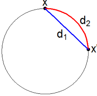
Figure 1: Chordal ( d_1 ) and geodesic ( d_2 ) distances on \mathbb{S} .
