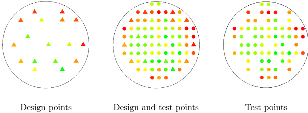
Figure 4: Color representation of thickness values. The 81 measurement locations are shown in the middle, including 17 design points (triangles, left) and 64 test points (bullets, right).
