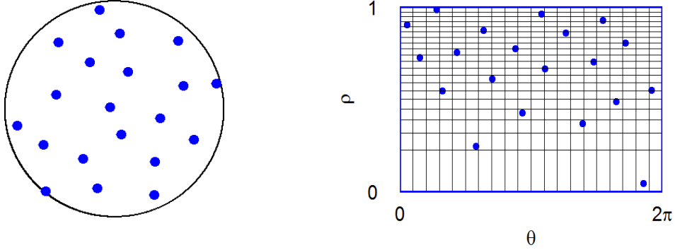
Figure 12: Cartesian (left) and polar (right) representations of the LCD obtained by transforming the maximin LCD of Figure 11 with \rho \mapsto \sqrt{\rho} .
