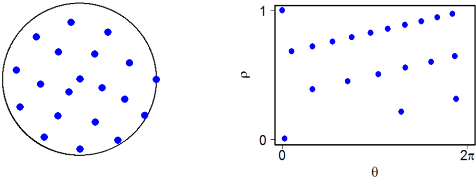
Figure 10: Cartesian (left) and polar (right) representations of the Archimedean spiral DoE. This DoE is filling well the disk but not the cylinder of polar coordinates.
