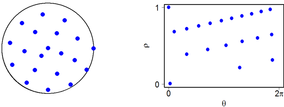
Figure 10: Cartesian (left) and polar (right) representations of the Archimedean spiral DoE. This DoE is filling well the disk but not the cylinder of polar coordinates.
