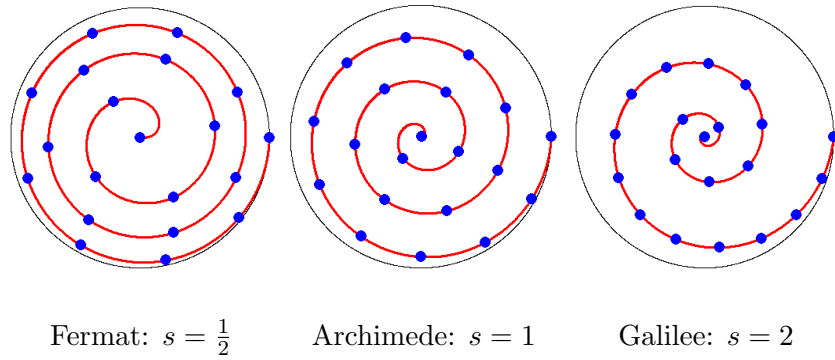
Figure 9: 20-point DoEs defined from spirals of the form \rho = a\theta^s + b with \theta \in [0, 6\pi] . The parameter s controls the speed with which the curve moves away from the center, and a, b are chosen such that the spirals start at the center and end at the boundary.
