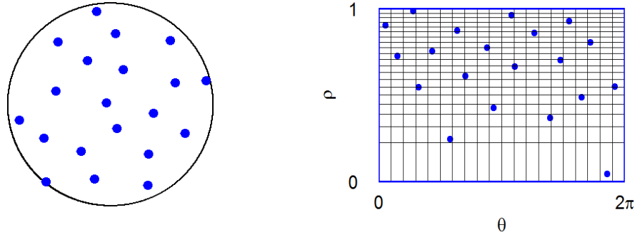
Figure 12: Cartesian (left) and polar (right) representations of the LHD obtained by transforming the maximin LHD of Figure 11 with \rho \mapsto \sqrt{\rho} .
