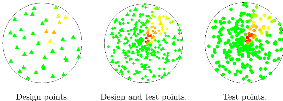
Figure 6: Color representation of gas concentrations. The 242 simulation locations are shown in the middle, including 30 design points (triangles, left) and 212 test points (bullets, right).
