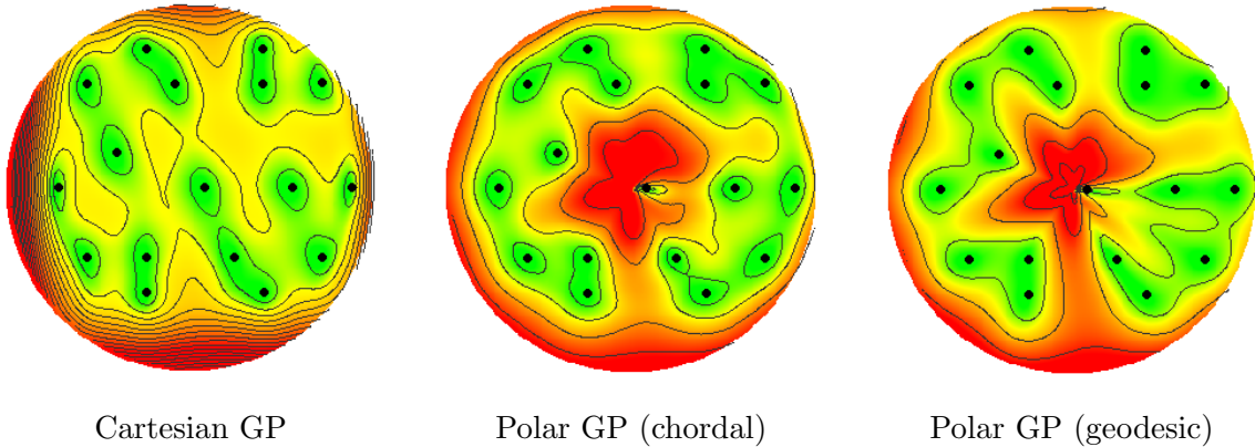
Figure 3: Kriging standard deviations for Cartesian and polar GPs (kernels (a)-(c))
