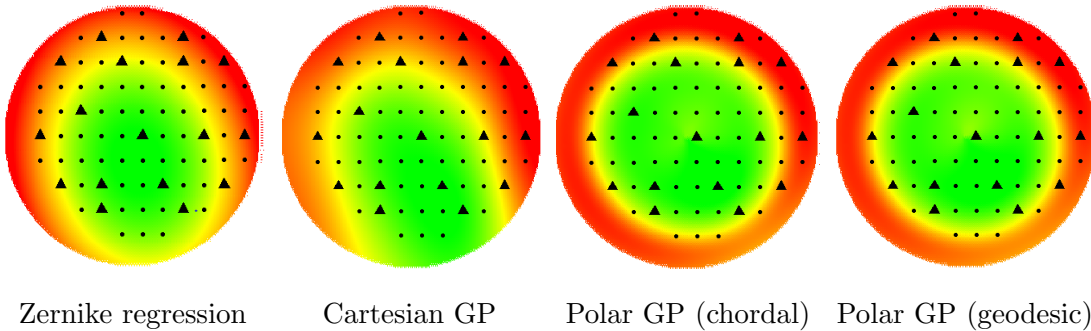
Figure 5: Prediction surface for the best untrended GP models of Table 1. When adding a Zernike trend, the prediction surface is approximately the same as for a pure Zernike regression represented on the left. Black bullets correspond to test points, triangles to design points.
