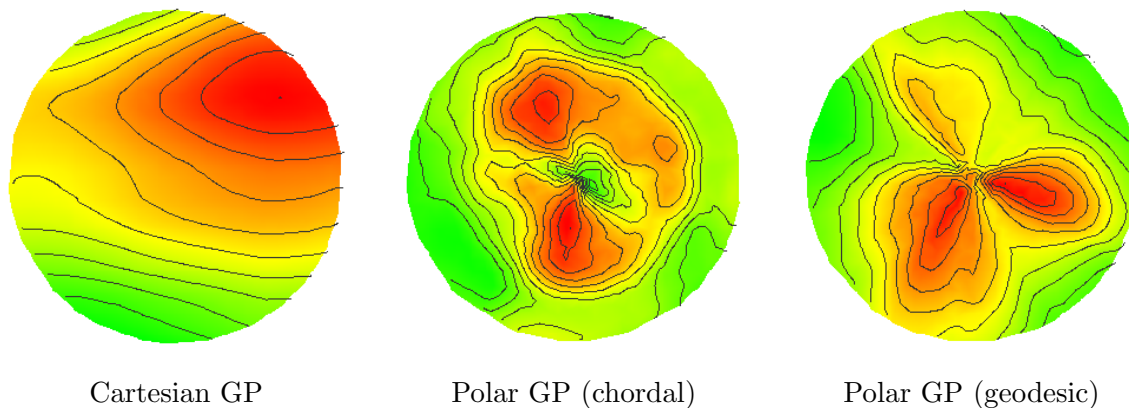
Figure 2: Simulations of Cartesian and polar GPs with kernels (a)-(c).
