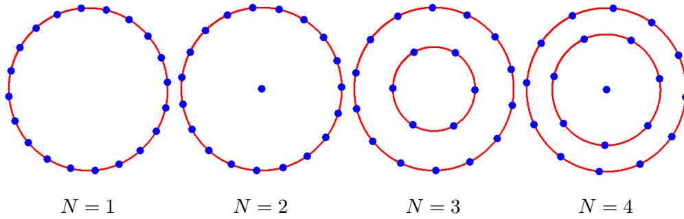
Figure 8: 20-point D-optimal DoEs for Zernike polynomials of degree N .
