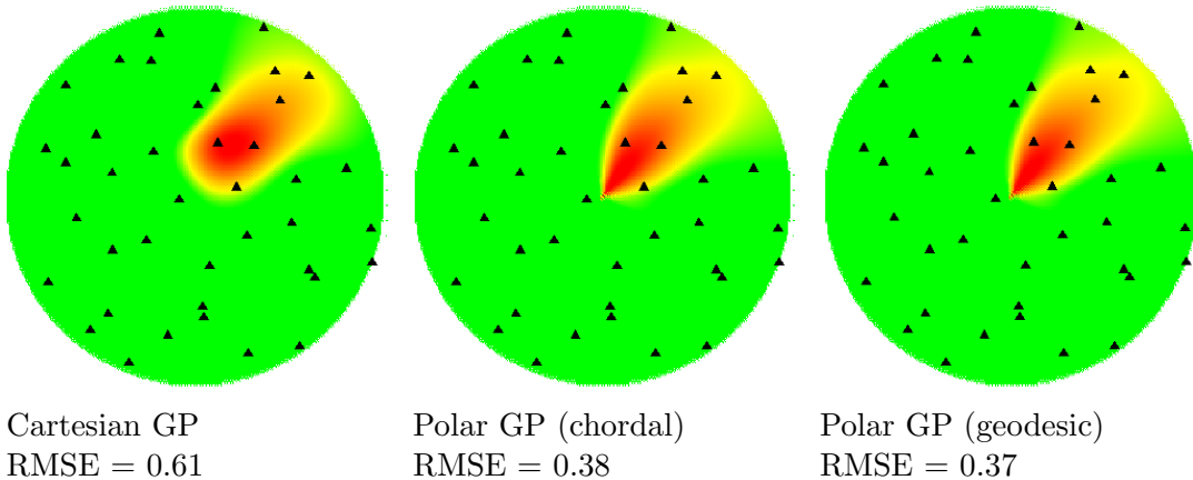
Figure 7: Estimated gas concentrations according to wind speed ( \rho ) and direction ( \theta ), for untrended Cartesian and polar GPs. Adding a Zernike polynomial trend does not improve the results. Triangles correspond to design points.
