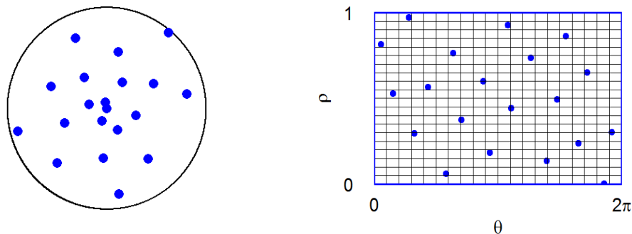
Figure 11: Cartesian (left) and polar (right) representations of a 20-point maximin LHD. The design is well-filling the cylinder \mathcal{C} of polar coordinates, displayed as a 2-dimensional map: In particular, the design points near the left and right boundaries are also spread out from each other.
