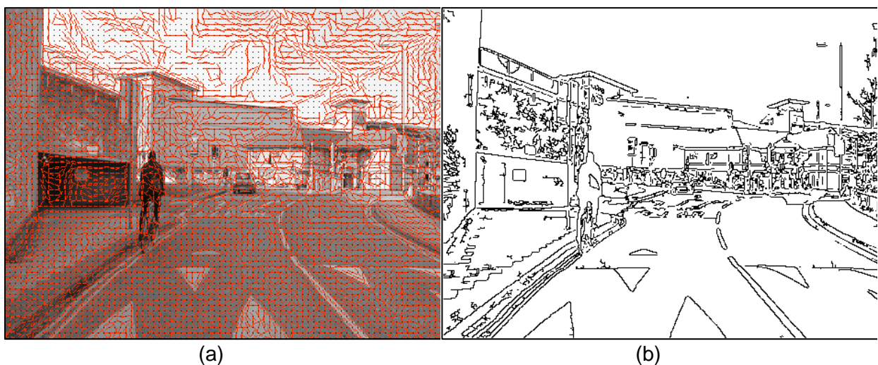
Figure 3: Two examples of contrast invariant features (a) Direction of the isophote (orthogonal to gradient), and (b) Contours defined as the local maxima of the gradient intensity in the gradient direction.
