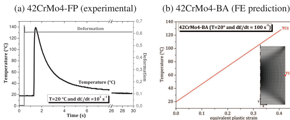
Figure 11: Increase of the temperature during deformation due to self-heating for a compression test at T = 20^{\circ}\text{C} and \dot{\epsilon} = 10^2 \text{ s}^{-1} . Comparison between (a) The experimental measurement the 42CrMo4-FP steel and (b) The FE prediction for the 42CrMo4-BA steel.
