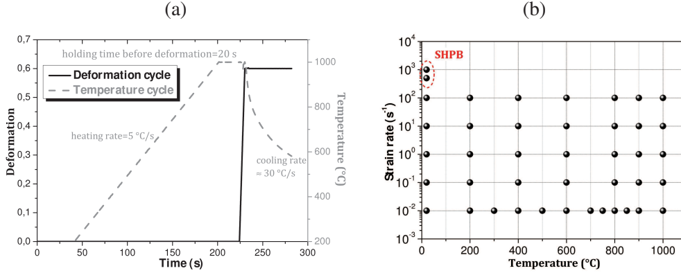
Figure 5: (a) Applied thermal-mechanical cycle, (b) the different test conditions investigated.
