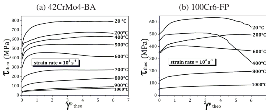
Figure 9: Evolution of the shear stress as a function of the plastic shear strain for (a) the 42CrMo4-BA steel and (B) the 100Cr6-FP steel, at different temperatures and an equivalent strain rate of 10^2 \text{ s}^{-1} .
