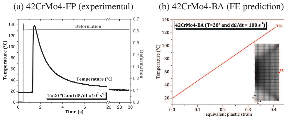
Figure 11: Increase of the temperature during deformation due to self-heating for a compression test at T = 20^\circ\text{C} and \dot{\epsilon} = 10^2 \text{ s}^{-1} . Comparison between (a) The experimental measurement the 42CrMo4-FP steel and (b) The FE prediction for the 42CrMo4-BA steel.
