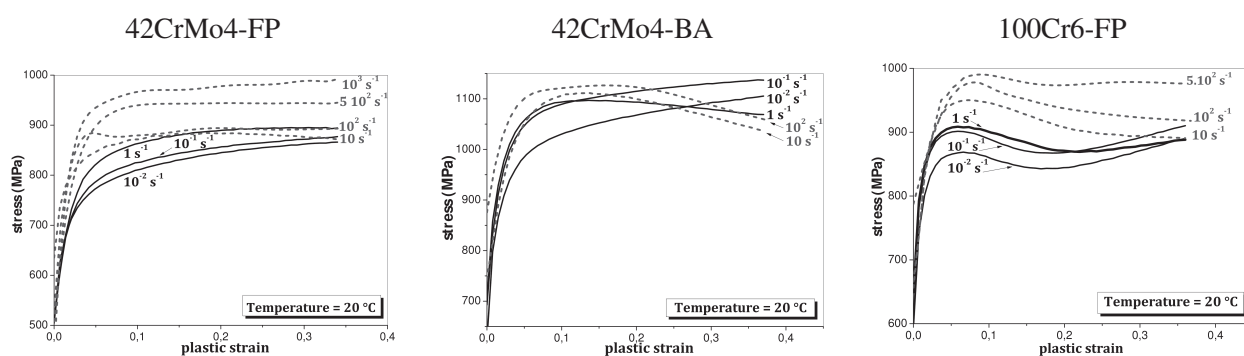
Figure 10: Evolution of the compressive stress as a function of the plastic strain at 20^\circ\text{C} for different strain rates. Comparison between the three steels studied.
