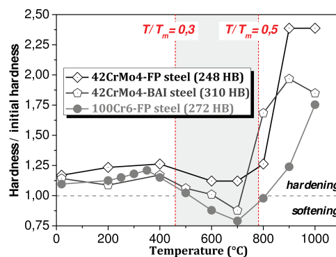
Figure 23: Hardness of the cylindrical specimens after testing at different temperatures and at a constant strain rate of ( 10^{-2} s^{-1} ) and for a constant strain of 0.6. Comparison between the three steels studied.
