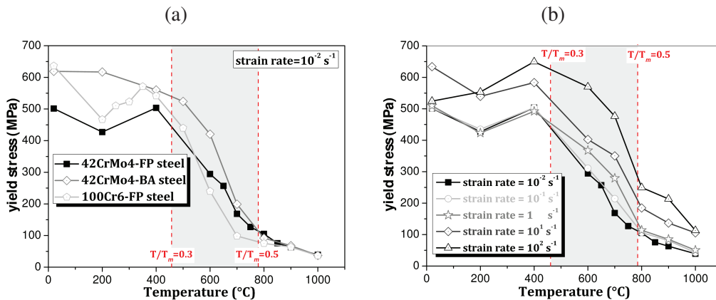
Figure 7: Evolution of the compressive yield stress as a function of the temperature (a) for the three steels investigated, and (b) for the 42CrMo4-FP steel, at different strain rates.
