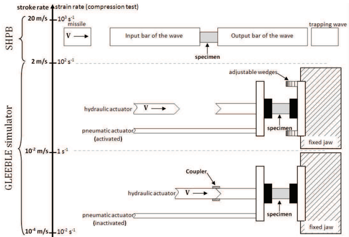
Figure 4: The three configurations used for compression (and shear) tests done using a GLEEBLE machine and a Split Hopkinson Pressure Bars apparatus.
