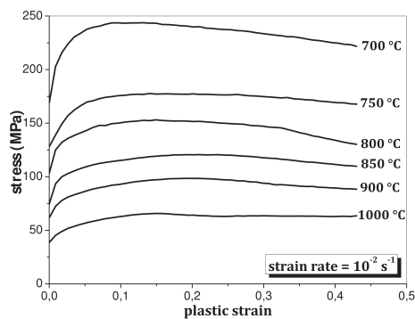
Figure 19: Evolution of the compressive stress as a function of plastic strain for a constant strain rate of ( 10^{-2} s^{-1} ) and for different temperatures close to the phase change temperature for the 42CrMo4-FP steel.
