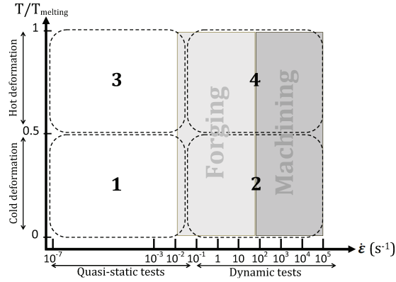
Figure 1: Imposed strain rate (in \text{s}^{-1} ) and temperature ranges in forging and machining operations and different domains of mechanical behaviour.
