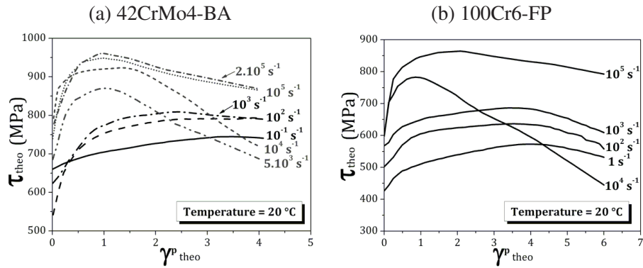
Figure 14: Evolution of the shear stress as a function of the plastic shear strain at 20°C for different equivalent strain rates, for steels (a) 42CrMo4-BA and (b) 100Cr6-FP.
