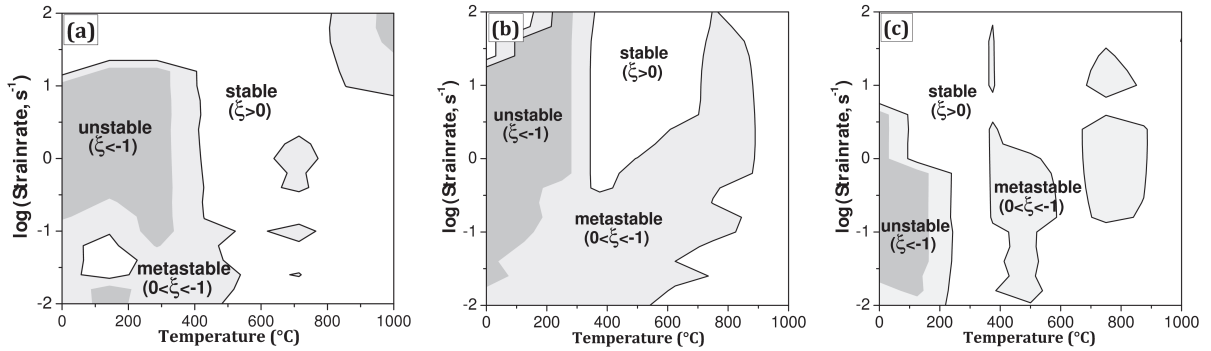
Figure 22: Unstable flow maps for the three steels investigated: (a) 42CrMo4-FP, (b) 42CrMo4-BA and (c) 100Cr6-FP.
