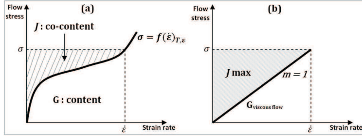
Figure 2: Schematic representation of (a) the content ( G ) and co-content ( J ) dissipated power for a material with a behaviour given by a curve \sigma = f(\dot{\epsilon}) (the total dissipated power is given by the rectangle) and (b) the maximum complementary dissipated power J_{max} obtained for a sensitivity to the strain rate m = 1 [9].
