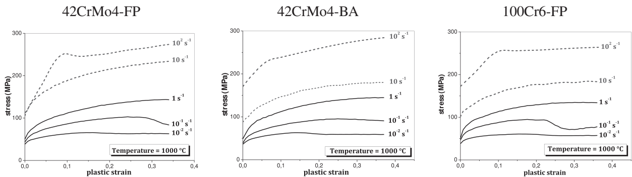
Figure 17: Evolution of the compressive stress as a function of the plastic strain at 1000°C for different strain rates. Comparison between the three steels studied.
