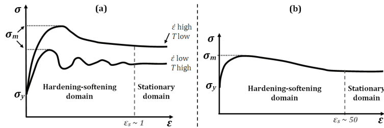
Figure 18: Characteristic stress-strain curves for a metal with (a) low stacking fault energy and (b) high stacking fault energy [4].
