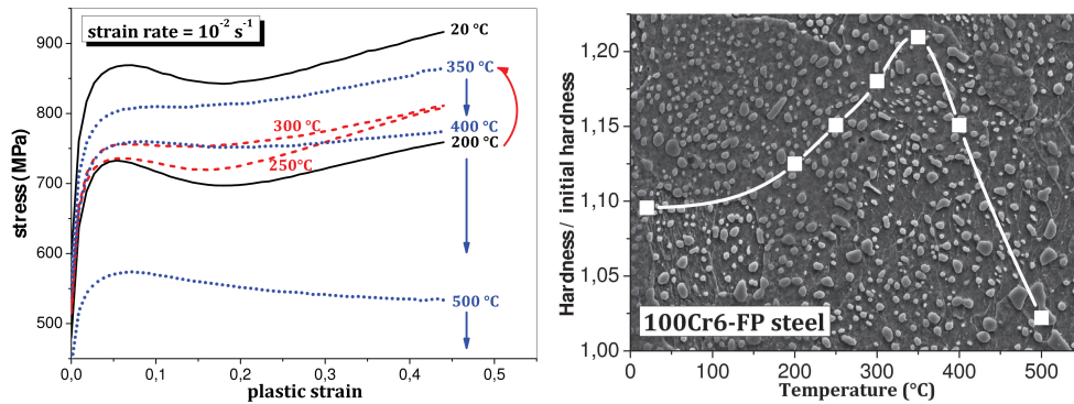
Figure 25: Behaviour curves for the 100Cr6 steel loaded in compression for a strain rate of \dot{\epsilon} = 10^{-2} \text{ s}^{-1} and for temperatures ranging from 20 to 500 °C and the hardness of the deformed specimens.
