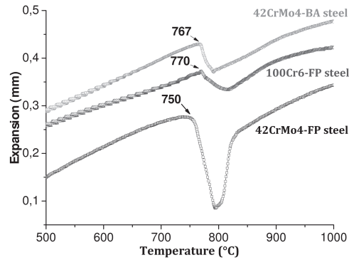
Figure 20: Evolution of the thermal dilation as a function of the temperature during the heating step.
