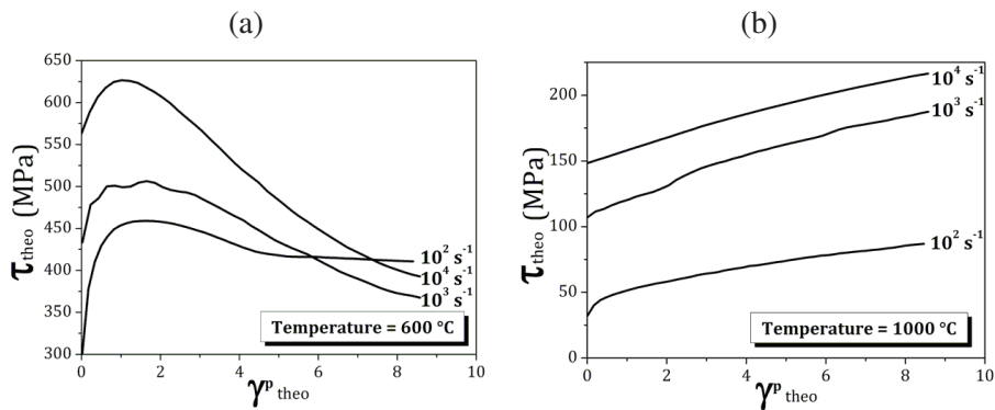
Figure 16: Evolution of the shear stress as a function of the plastic shear strain at (a) 600°C and (b) 1000°C for different equivalent strain rates for the steel 42CrMo4-BA.
