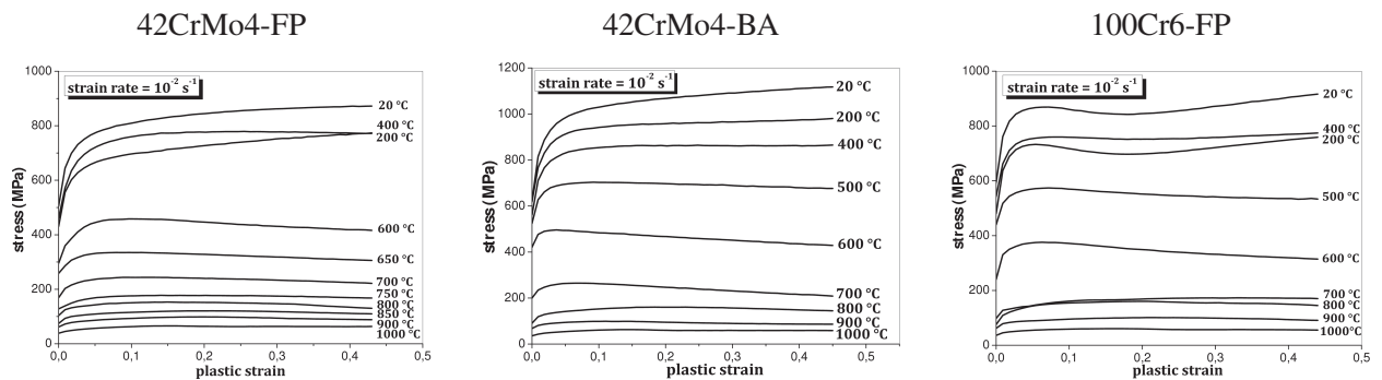
Figure 8: Evolution of the compressive stress as a function of plastic strain for the three steels investigated at different temperatures and at a strain rate of 10^{-2} \text{ s}^{-1} .
