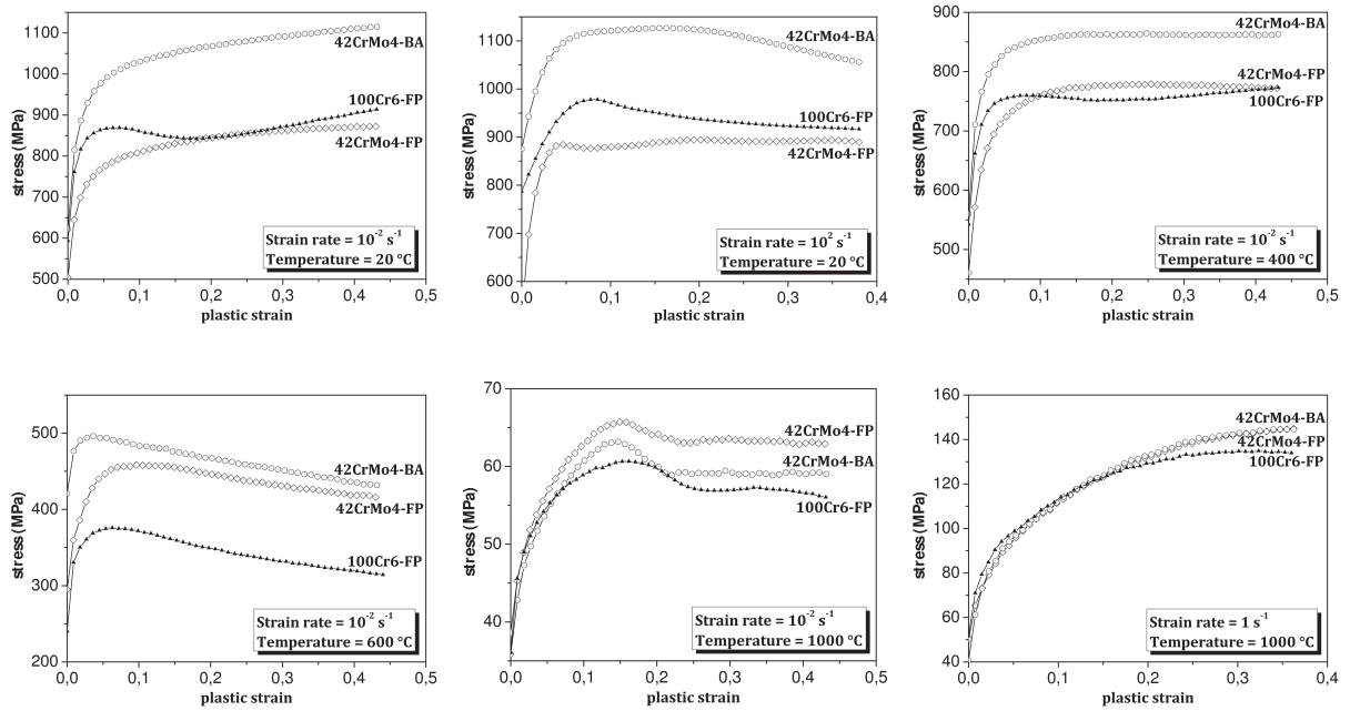
Figure 26: Comparison of the shape of the stress-plastic strain curves for three steels studied in the three deformation domains.
