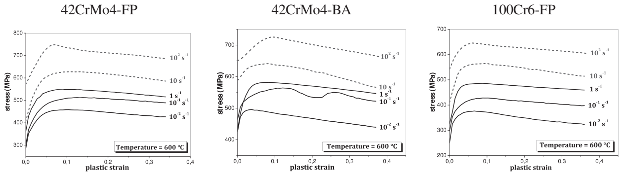
Figure 15: Evolution of the compressive stress as a function of the plastic strain at 600°C for different strain rates. Comparison between the three steels studied.
