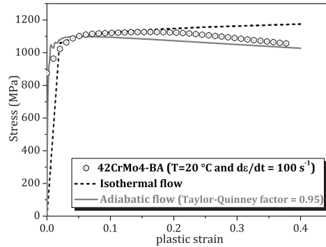
Figure 13: Comparison between the stress-strain curves for the case of adiabatic flow (with a Taylor-Quinney factor = 0.95) and isothermal flow for the 42CrMo4-BA steel at T = 20^{\circ}\text{C} and \dot{\epsilon} = 10^2 \text{ s}^{-1} .
