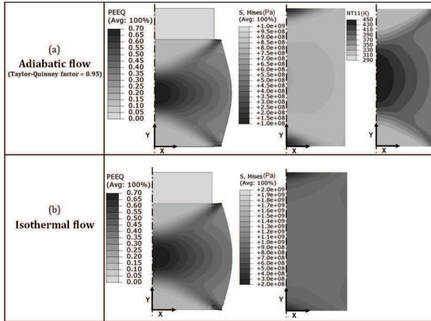
Figure 12: Comparison between equivalent strain, temperature and equivalent stress maps obtained by FE calculation with Abaqus Explicit for (a) adiabatic flow and (b) isothermal flow.
