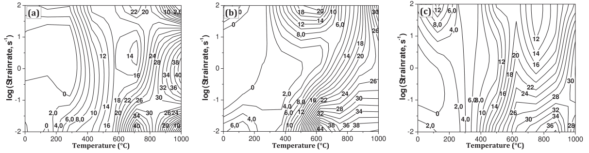
Figure 21: Efficiency maps (in %) for the three steels studied: (a) 42CrMo4-FP, (b) 42CrMo4-BA and (c) 100Cr6-FP.
