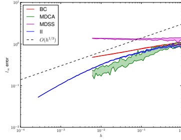
(e) Flower- \hat{\kappa}_R - l_\infty
