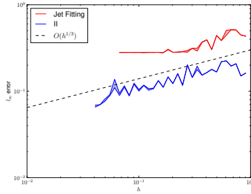
(h) RoundedCube- \hat{\kappa}_R^2-l_\infty
