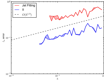
(e) RoundedCube- \hat{\kappa}_R^1-l_\infty
