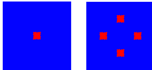
Fig. 3 Initial condition for the cell density u (left) with 0 \leq u \leq 1 and for the chemoattractant concentration v (right) with 0 \leq v \leq 5 .
