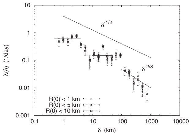
FIG. 9. FSLE for R(0) \leq 1, \leq 5 , and \leq 10 km and amplification factor \rho = \sqrt{2} . The small-scale plateau corresponds to exponential separation with rate \lambda_L \simeq 0.6 \text{ day}^{-1} . The \sim \delta^{-2/3} scaling corresponds to the Richardson law. The \delta^{-1/2} scaling corresponds to a k^{-2} spectrum. Error bars are the standard deviations of the mean values.
