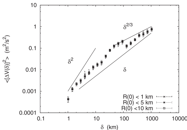
FIG. 10. FSRV computed together with the FSLE. The FSRV is the mean exit velocity of the distance between two drifters from the “shell” \delta . The scalings \delta^2, \delta^{2/3} , and \delta correspond to k^{-3}, k^{-5/3} , and k^{-2} energy spectra, respectively. Error bars are the standard deviations of the mean values.
