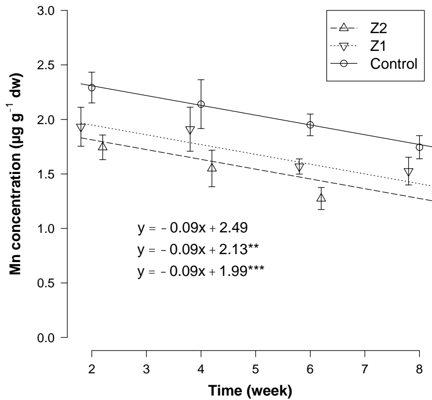
Figure 3: Total Mn concentrations (mean \pm SD; \mu\text{g g}^{-1} dw) in juvenile cuttlefish reared in control and in two Zn concentrations (Z1, Z2). Asterisks correspond to significant differences compared to control (** < 0.01 , *** < 0.001 ).
