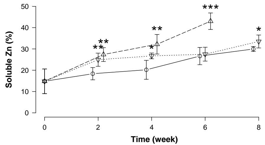
Figure 4: Soluble Ag, Cd, Cu and Zn proportions (mean \pm SD; %) in juvenile cuttlefish reared in control and in 2 Zn concentrations (Z1, Z2). Asterisks correspond to significant differences compared to control (* < 0.05, ** < 0.01, *** < 0.001).
