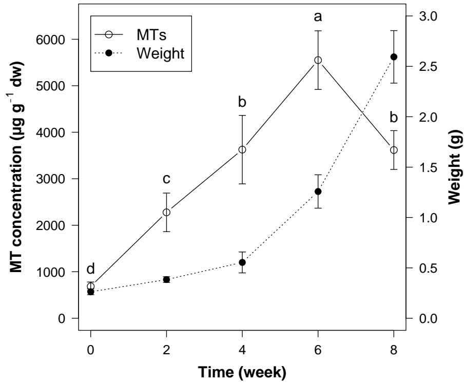
Figure 1: Metallothionein concentrations (mean \pm SD; \mu\text{g g}^{-1} dw) in juvenile cuttlefish and associated weight (mean \pm SD; g) during the 2 months post-hatching. Letters above the metallothionein concentrations indicate significant differences between groups ( p -value < 0.05).
