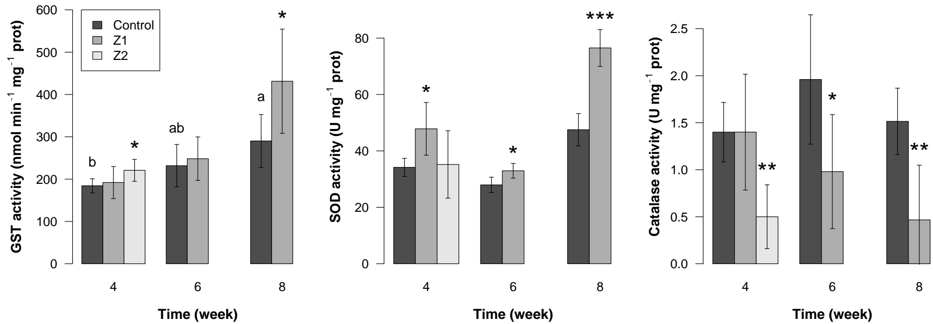
Figure 6: Glutathione S-transferase, superoxide dismutase and catalase activities (mean \pm SD; respectively in \text{nmol min}^{-1} \text{mg}^{-1} \text{prot} , \text{U mg}^{-1} \text{prot} , and \text{U mg}^{-1} \text{prot} ) in the digestive gland of juvenile cuttlefish in control, Z1 and Z2 conditions after 4-week post-hatching and in control and Z1 conditions after 6- and 8-week post-hatching. Letters above control indicate its change over time, and asterisks above Z1 or Z2 correspond to significant differences of activity compared to control (* < 0.05 , ** < 0.01 ).
