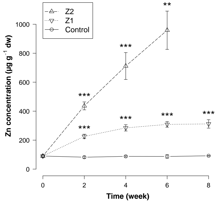
Figure 2: Total Zn concentrations (mean \pm SD; \mu\text{g g}^{-1} dw) in juvenile cuttlefish reared in control and in 2 Zn concentrations (Z1, Z2). Asterisks correspond to significant differences compared to control (* < 0.05 , ** < 0.01 , *** < 0.001 ).
