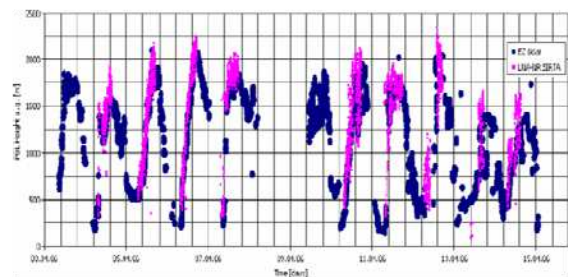
Fig. 2. PBL Height retrieval from EZLIDAR (blue) and STRAT (purple).
