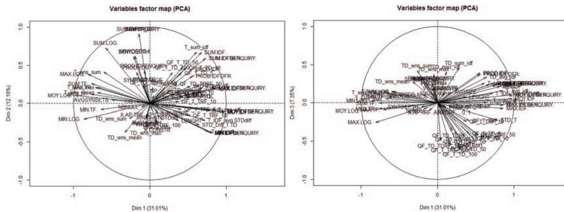
Fig. 3. Variables in the three dimensions of the PCA: dim1/dim2 on the left, dim1/dim3 on the right.
