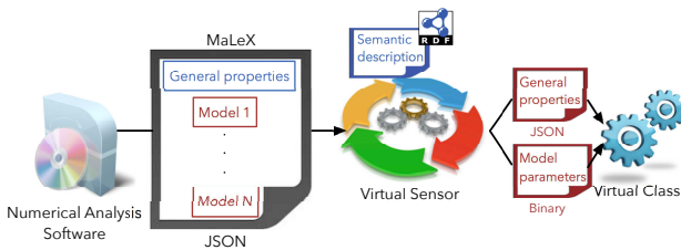
Figure 3: Model exchange between the different entities.
