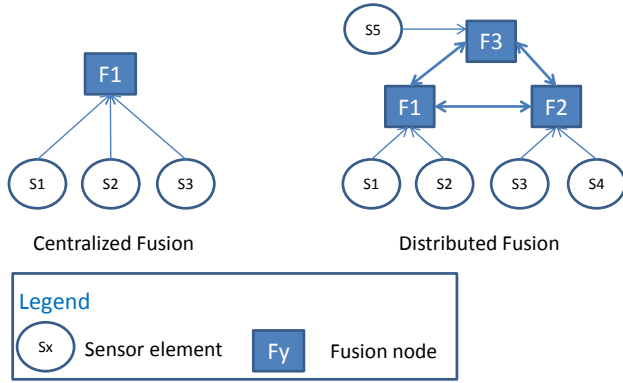
Fig. 5. Information graphs for centralized and fully distributed fusion architectures [13]
