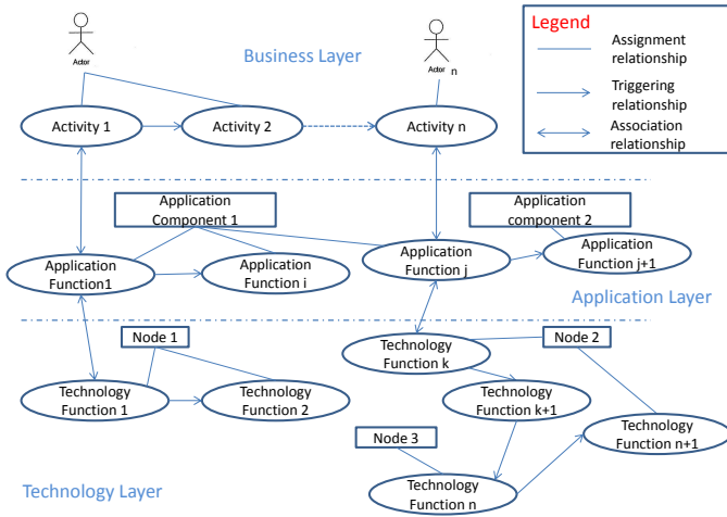
Fig. 4. A simplified example of multi-layered architecture of ArchiMate
