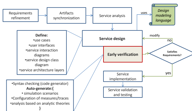
Fig. 1. Our approach: Extending the design activity by early verification in the service development framework, inspired from [1]
