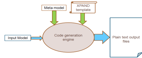
Fig. 3. XPAND workflow engine [10]
