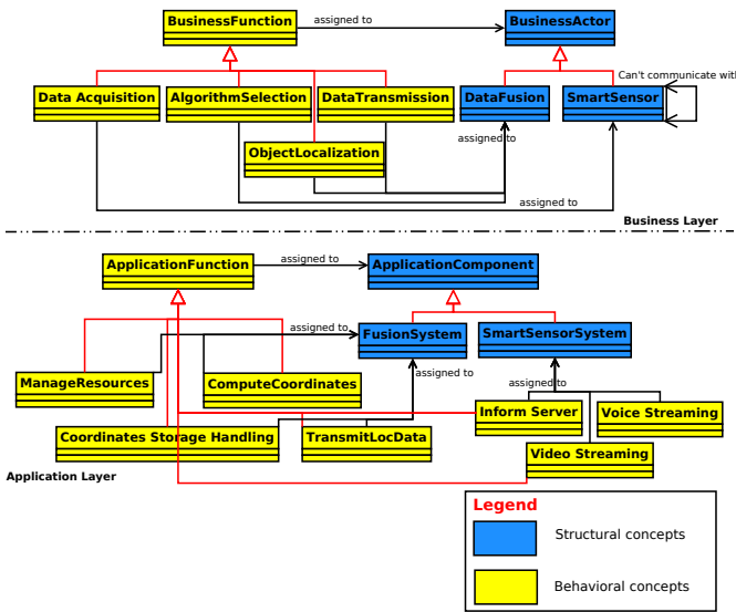
Fig. 6. Extending business and application layers of ArchiMate: proposal of DSO Meta-Model
