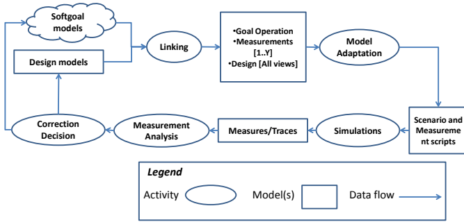
Fig. 2. Verification Activities in our approach [12]
