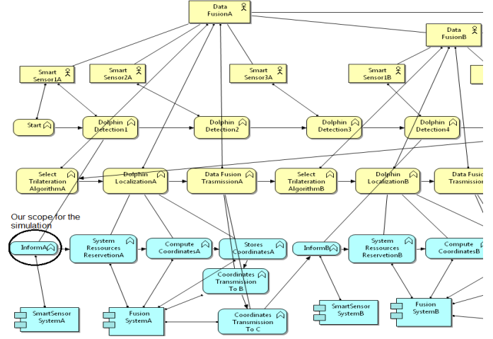
Fig. 7. Part of the model of an underwater localization, done by design tool that extends Archi. Layers are: Business and Application
