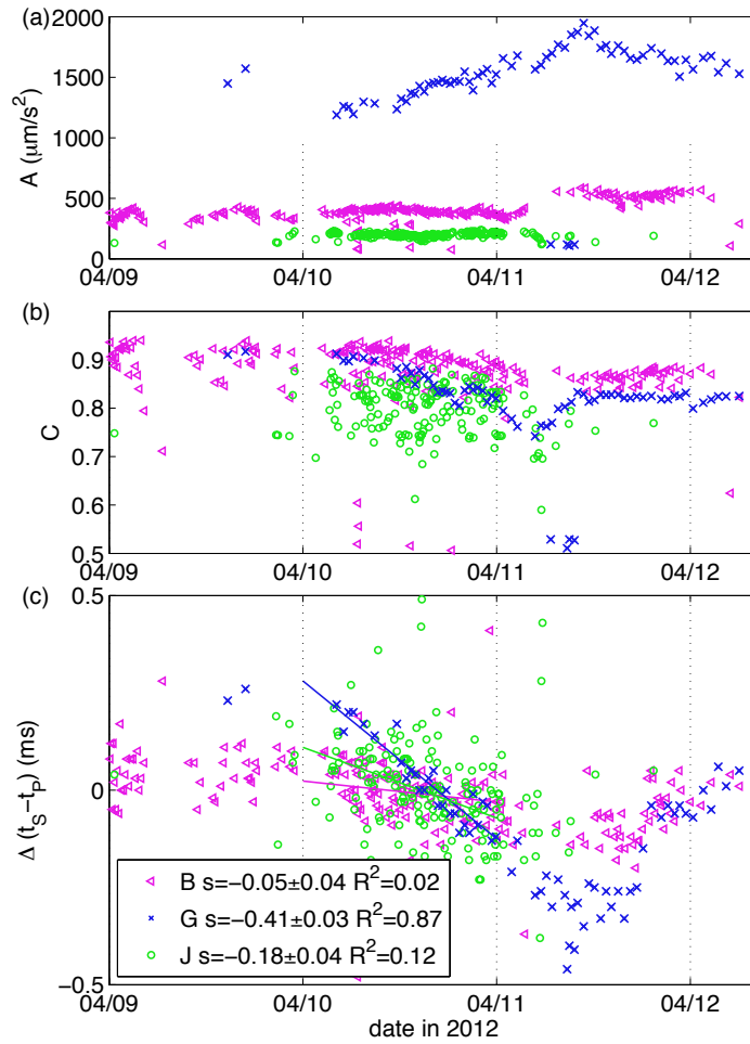
Figure 13: Temporal variations of the peak amplitude A (a), correlation with the template (b), and relative time delay between the P-waves and S-waves (c), for multipliers B , G and J . Solid lines in (c), linear fits for each multiplier using only the events that occurred on April 10. The slope (in ms/day) and its uncertainty (one standard error), and the correlation coefficient R^2 , are shown.
