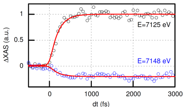
Figure 5. Time resolved change of X-ray absorption at 7125eV and 7148eV. Red lines are fit to single exponential rise with time constant \tau_{\langle \text{Fe-N} \rangle} = 170(20) fs. Adapted with permission from ref. 33. Copyright (2014) American Physical Society.
