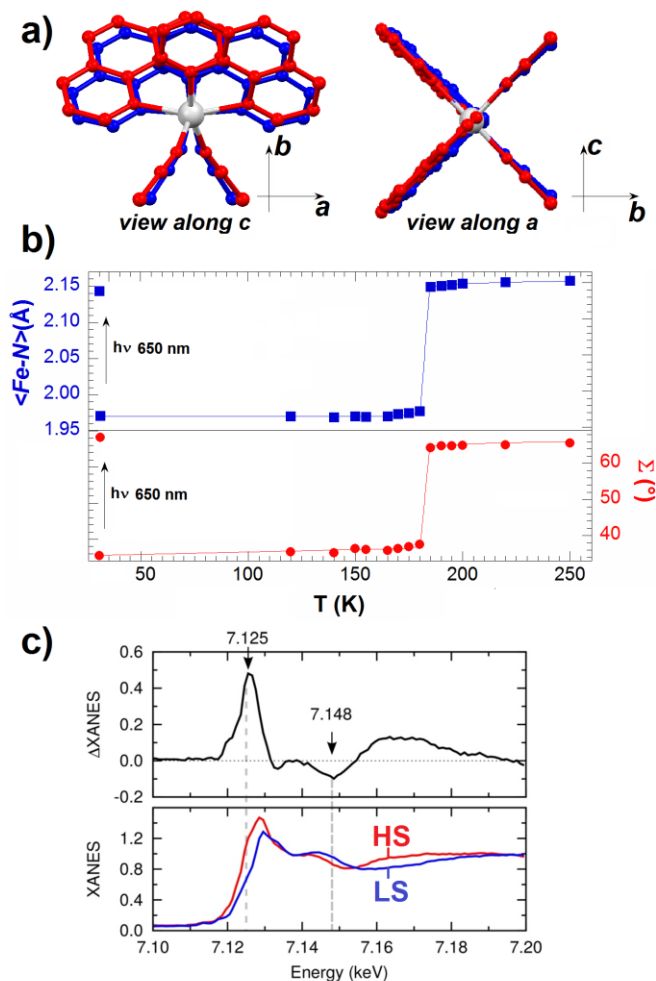
Figure 3. (a) LS (140 K, blue) and HS (200 K, red) structures of [\text{Fe}(\text{phen})_2(\text{NCS})_2] . (b) Temperature dependence of \text{Fe-N} bonds and \Sigma parameter, showing the first-order phase transition around 180 K between LS and HS states. The parameters obtained after cw irradiation at 650 nm are identical to those of the HS state at high temperature. (c) XANES spectra and variation \Delta\text{XANES} measured between the HS (200K) and LS (140K) states. Adapted with permission from ref. 33. Copyright (2014) American Physical Society.
