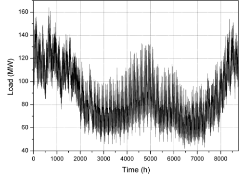
Figure 1: Load of the Perpignan grid in 2006
