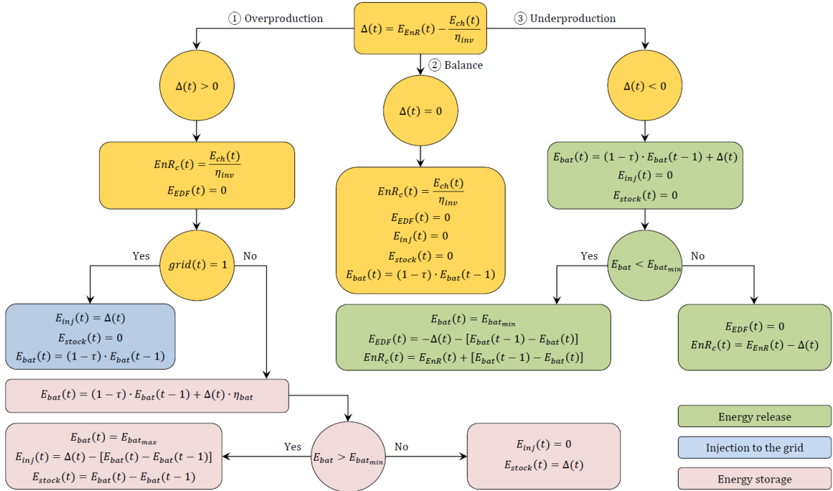
Figure 2: Energy management algorithm (see sections "Performance criteria" and "Batteries modelling")
