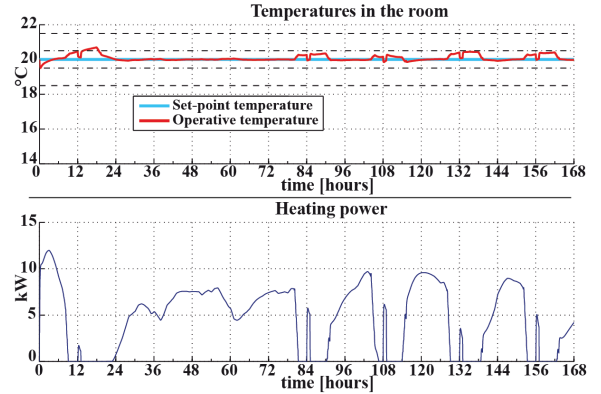
Figure 5: Temperatures and power for PI-S1
