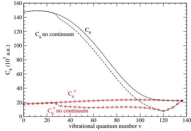
FIG. 8. (Color online) Same as Figure 7 for the C_6^e (circles) and C_6 (no symbols) coefficients.
