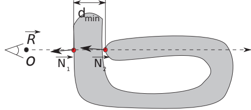
Figure 7: Calculation of d_{min} , which holds the minimum distance between surface points bound to two adjacent pixels to be used for crack pixel detection. B-Rep models identify solid models and only their exterior, front-facing faces are visible and therefore rendered. d_{min} can be set to the minimum possible distance travelled by a single ray (dotted line) intersecting the B-Rep model at front-facing locations (red) with respects to the observer (left).
