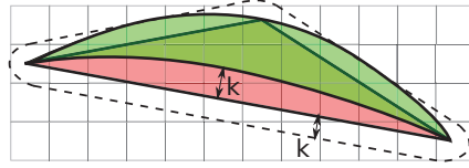
Figure 5: The red triangle is a k -pixel approximation of the B-Rep surface (green) section it represents. The k -pixel covering accuracy defined by Yeo et al. guarantees that the B-Rep surface footprint on screen is located within the k -pixel sized ring (dashed line) around the triangle.
