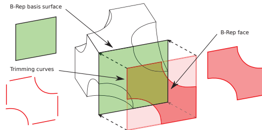
Figure 2: Anatomy of a B-Rep model face.
