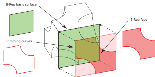
Figure 2: Anatomy of a B-Rep model face.
