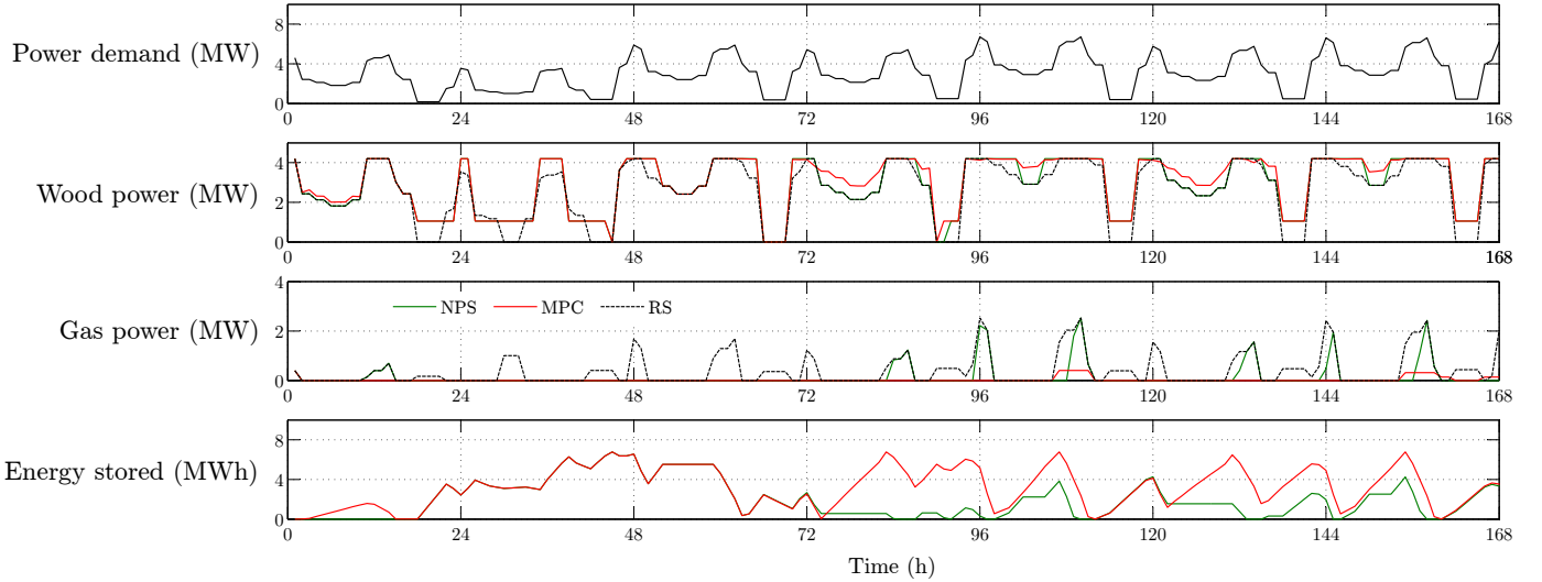
Fig. 4. Weekly dynamics of the multi-energy district boiler.
