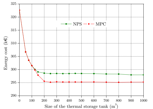
Fig. 6. Impact of the size of the tank on Ec .
