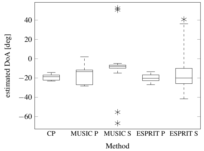
Figure 6: DoA estimation throughout the cluster of deep events
