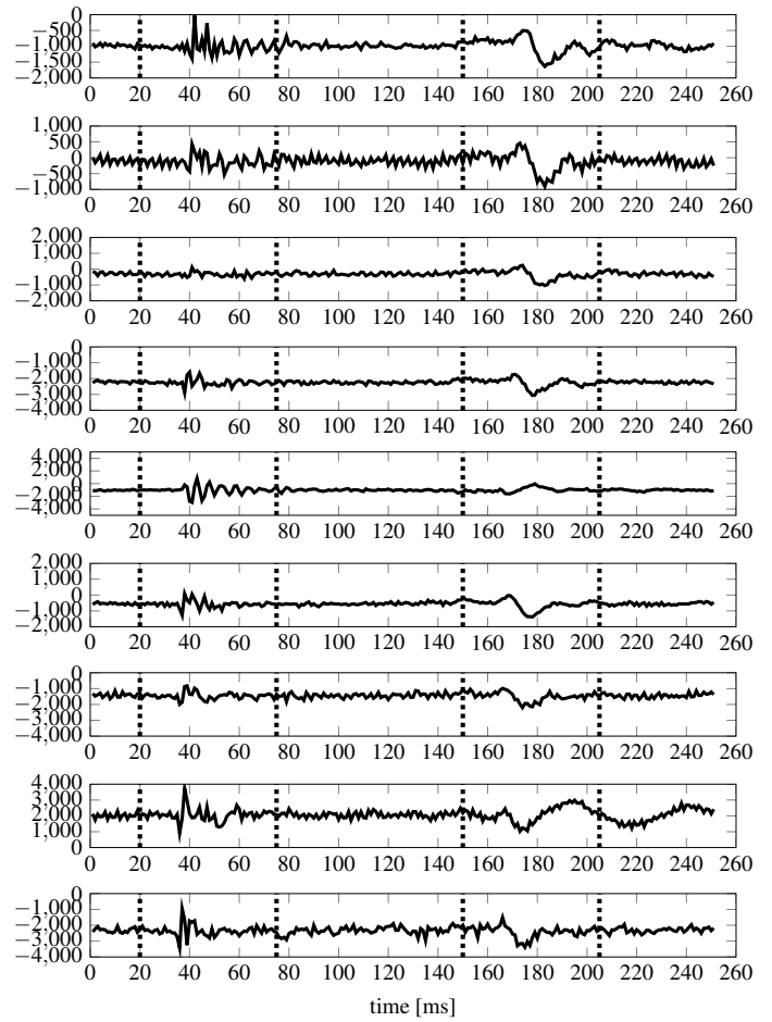
Figure 7: Example of an event from the Argentière glacier - 2012: record from the array with distinct P and S waves - vertical component
