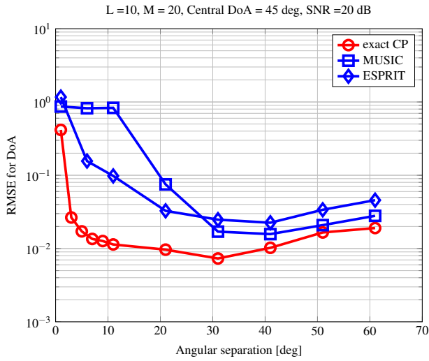
Figure 3: RMSE [rad] vs angular separation [deg] - endfire perspective
