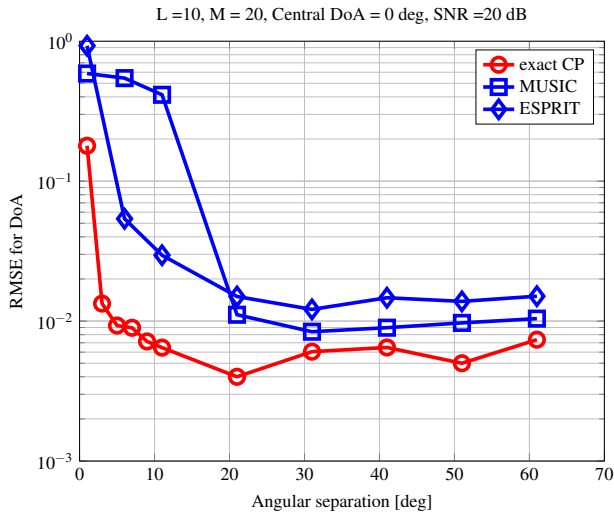
Figure 4: RMSE [rad] vs angular separation [deg] - broadside perspective
