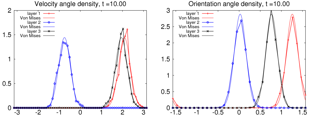
Figure 2: (Homogeneous case, non-interacting layers) Left: Distributions of velocity angle \varphi at time t = 10 . Right: Distributions of inclination angle \theta at time t = 10 . Numerical parameters: \nu = 4 , D = 0.3 , K = 4 , \delta = 0.3 , \Delta t = 10^{-2} . Number of particles: 600 per layer.
