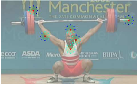
Fig. 5. SMP^{u2} configurations allow to determine the shape of the rigid parts of the moving object around the keypoints (in red points). In the neighbouring circles, image patches in green (resp. blue) indicates that they belong to the same rigid part of the moving object as the keypoint (resp. another rigid part or the background).
