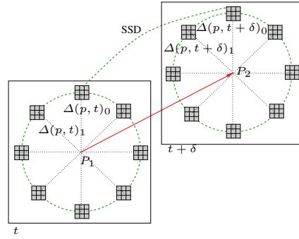
Fig. 4. The SMP descriptor is calculated at each tracked keypoint, along its trajectory. The consistency of motion in every direction is checked by computing the SSD between the corresponding image patches.
