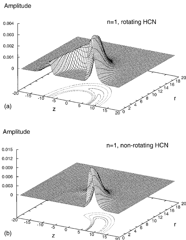
FIG. 2. Two-dimensional representation of the ground state wave function \Psi of the HCN-He n=1 dimer. \Psi was computed with unbiased DMC here. The rotation of the HCN molecule is included in (a), whereas (b) corresponds to a nonrotating (but translating) HCN molecule. The origin is set at the molecular center of mass. The HCN molecule is oriented as N-C-H, the H atom being at positive z . All distances are in atomic units. The normalization of the amplitude is arbitrary but identical in both figures.
