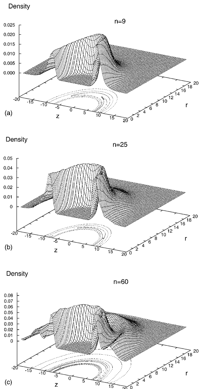
FIG. 3. Ground state helium density for: (a) HCN He _9 , (b) HCN He _{25} , (c) HCN He _{60} . The mixed densities are shown here, i.e., \rho_{\text{mixed}} = \langle \Psi | \hat{\rho} | \Psi \rangle . The orientation of the HCN molecule is identical to that defined in Fig. 2.
