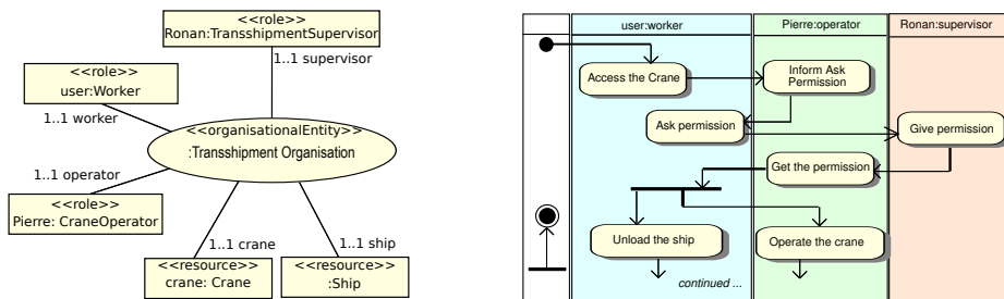
Fig. 3. Modelling of the transshipment activity using HAVE (partial).
