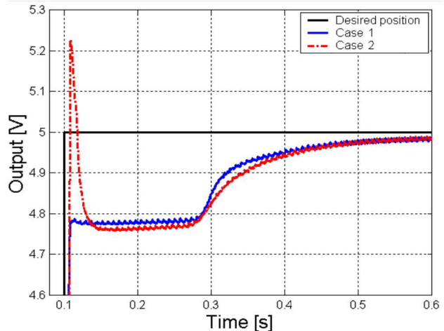
Fig. 1. Stick-slip phenomenon on a pneumatic cylinder.
