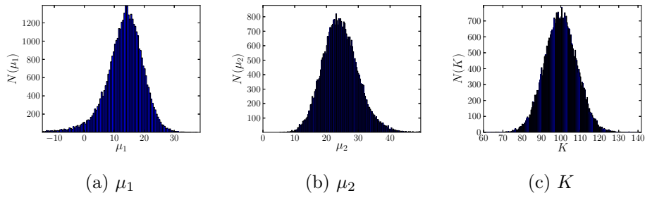
Figure C.10: Histograms (number of counts) of the measured values of the local elastic constants \mu_1 , \mu_2 , and K in subregions of size 5\sigma_{AA} \times 5\sigma_{AA} in the MD system.
