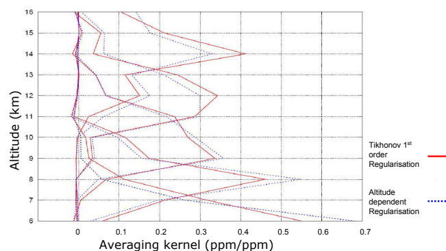
Fig. 4b. Averaging kernels for levels at 6, 8, 10, 12, and 14 km for one occultation. The red curve corresponds to a first order Tikhonov regularisation and the blue curve to an altitude dependent regularisation based on a Tikhonov first order operator.
