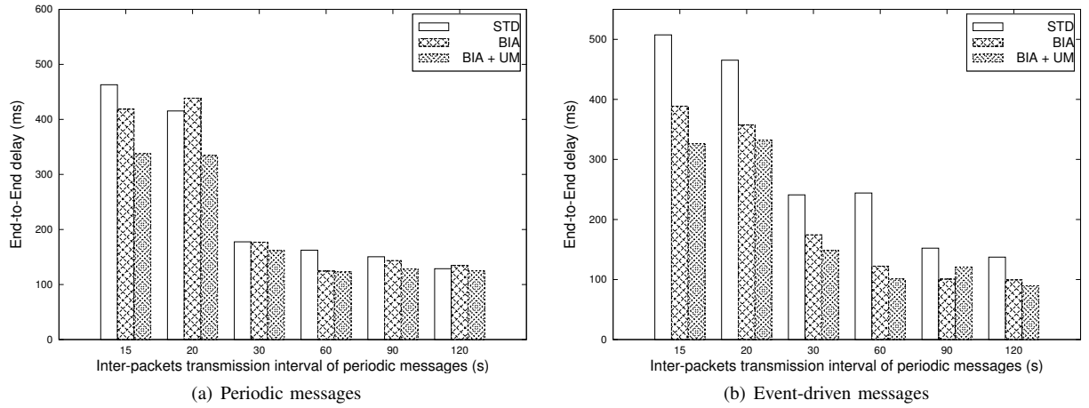
Figure 8: Impact of inter-packets transmission interval on Average End-to-End delay: Proportion of event driven messages=4%, Network size=50
