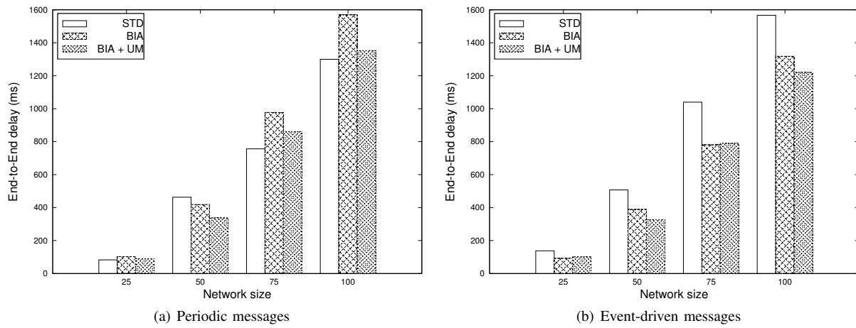
Figure 10: Impact of Network size on Average End-to-End delay: Proportion of event-driven messages = 4%, Inter-packets transmission interval = 15 s
