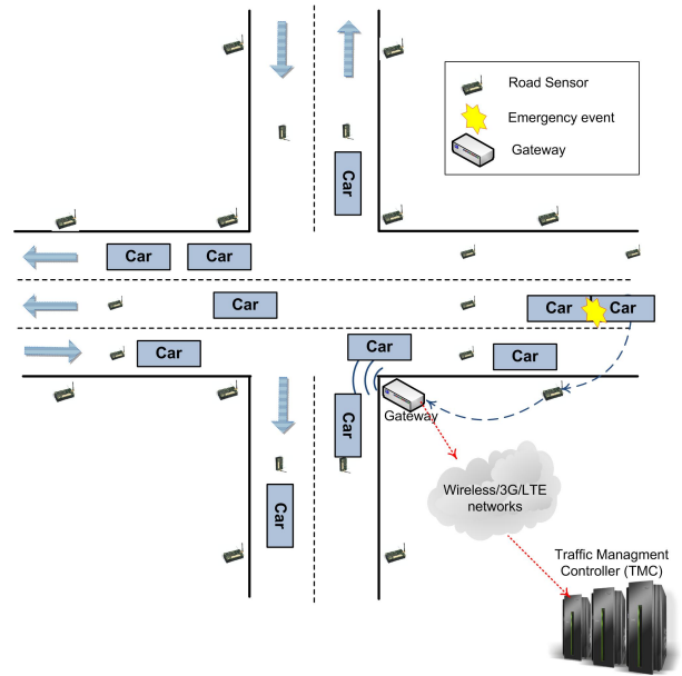
Figure 1: WSNs deployed in road networks for traffic flow monitoring and emergency events detection and reporting
