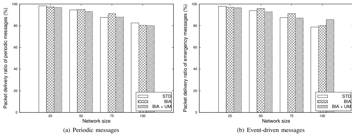
Figure 11: Impact of Network size on Packets Delivery Ratio: Proportion of event-driven messages = 4%, Inter-packets transmission interval = 15 s
