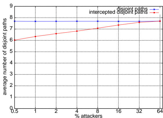
Figure 10. Average number of disjoint paths (total and intercepted) per source-destination pair in ER 20k-node networks.
