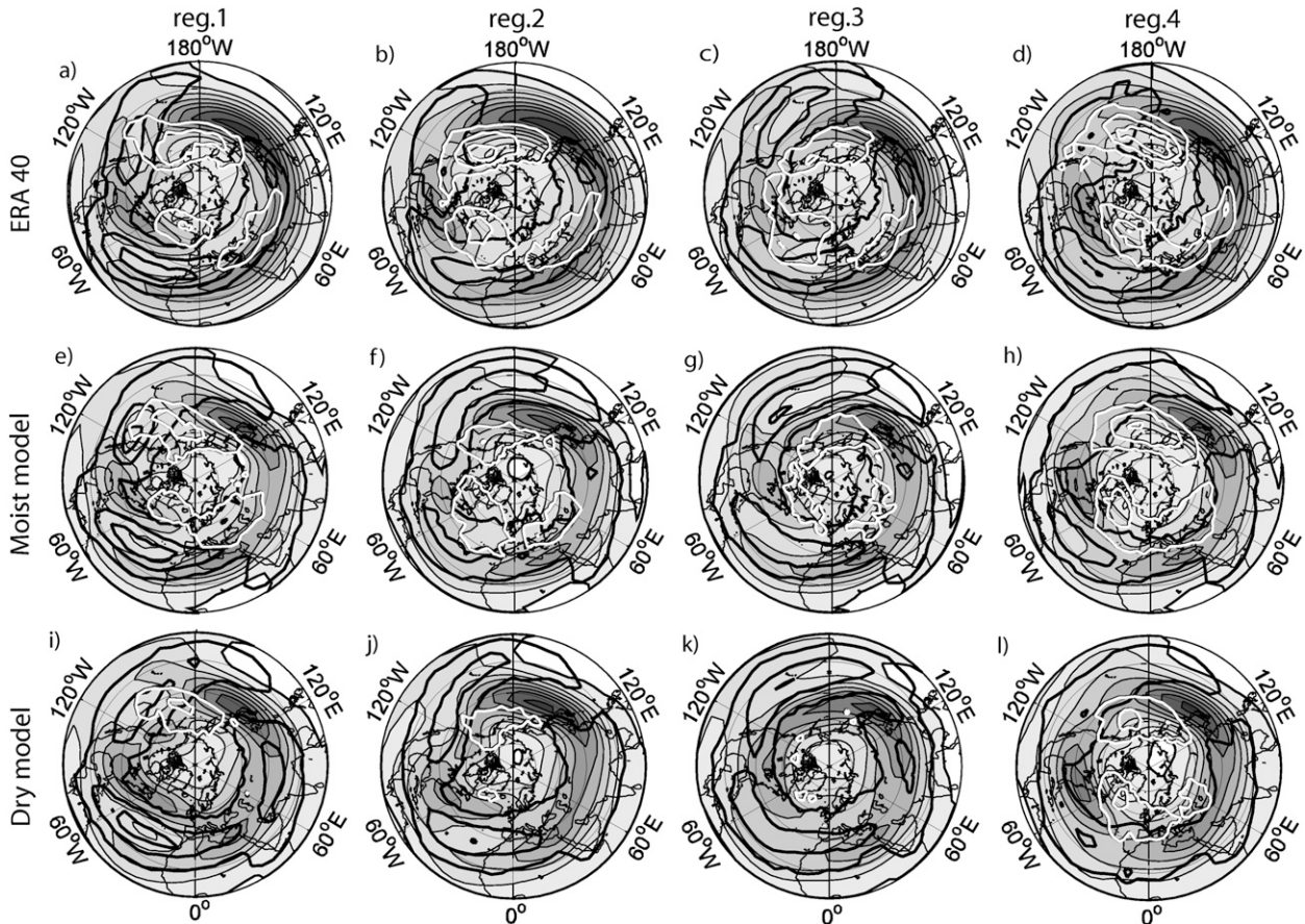
FIG. 8. Composite of the 200-hPa zonal wind speed (gray shading with contours every 10 \text{ m s}^{-1} ), AWB (thick black contours every 0.1 \text{ day}^{-1} ), and CWB (white contours every 0.05 \text{ day}^{-1} ), associated with the regimes presented in Fig. 4, for (a)–(d) ERA-40, (e)–(h) the moist model, and (i)–(l) the dry model.
