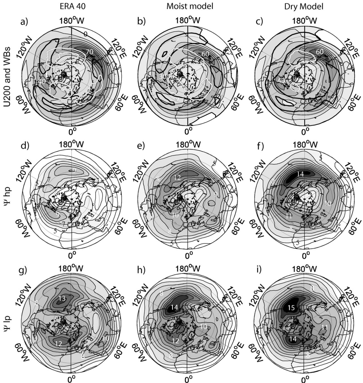
FIG. 2. (a)–(c) Zonal wind ( \text{m s}^{-1} ) and wave breaking frequencies of occurrence for AWB (black contours every 0.1 \text{ day}^{-1} ) and CWB (white contours every 0.05 \text{ day}^{-1} ) at 200 hPa for (a) ERA-40 (DJF 1967–2001), (b) the moist model, and (c) the dry model. (d)–(i) Standard deviation of the variability of the streamfunction ( \text{m}^2 \text{ s}^{-1} ), vertically averaged (using 800-, 500-, and 200-hPa levels), for (d),(g) ERA-40 and (e),(h) the moist and (f),(i) the dry versions of the model, for (d)–(f) synoptic-scale variability and (g)–(i) low-frequency variability.
