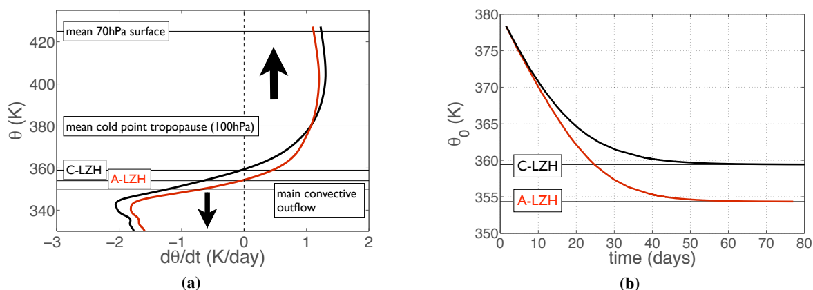
Fig. 1. (a) Annual mean tropical radiative heating rates ( 30^\circ\text{S} – 30^\circ\text{N} ) represented as change in potential temperatures, calculated for all-sky (in red) and clear-sky (in black) conditions, using the ERA-Interim dataset for 2005. (b) Time for transport from a source level, \theta_0 , to 380 K, calculated using the profiles shown in (a).
