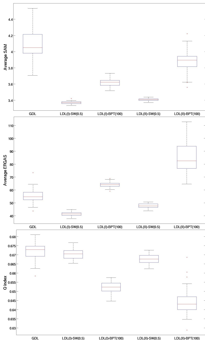
Fig. 11. Reconstruction errors for the Paris dataset using the estimated spectral response matrix [16]. The global approach (GDL) is compared to the proposed local approaches LDL(I) and LDL(II): (top) Average SAM, (middle) Average ERGAS and (bottom) UIQI index.
