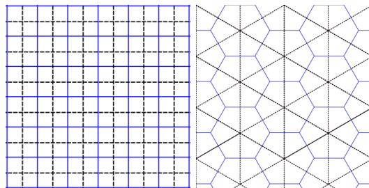
Figure 1: A square mesh and its dual (left), and a hexagonal mesh, in solid blue, and its dual mesh, the triangular tessellation, in dashed black (right).
