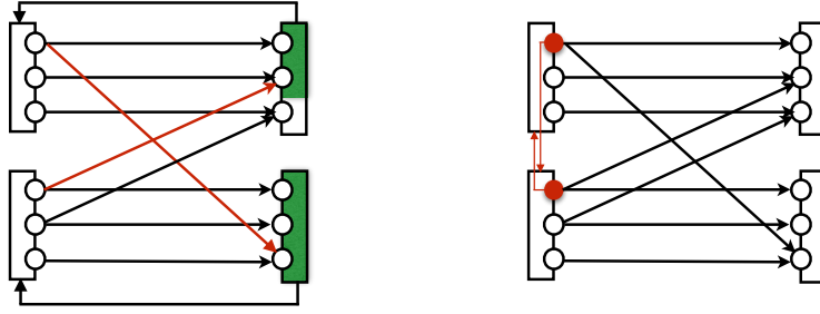
Figure 23: Source Cooperation vs Noisy Channel-Output Feedback.
