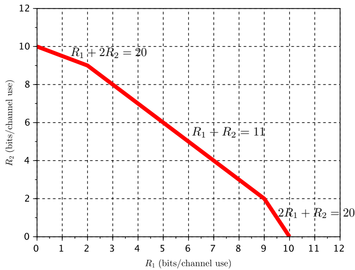
Figure 6: Capacity region of the example in Sec. 3.2.2 without feedback \mathcal{C}(10, 10, 3, 8, 0, 0)
