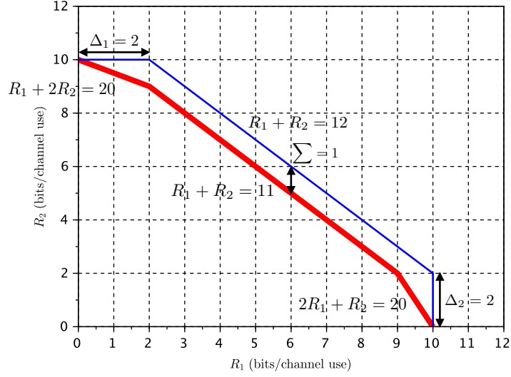
Figure 8: Capacity region \mathcal{C}(10,10,3,8,0,0) without feedback (thick red line) and \mathcal{C}(10,10,3,8,10,10) with perfect channel-output feedback (thin blue line) of the example in Sec. 3.2.2. Note that \Delta_1(10,10,3,8,10,10) = 2 bits/ch.use, \Delta_2(10,10,3,8,10,10) = 2 bits/ch.use and \Sigma(10,10,3,8,10,10) = 1 bit/ch.use.
