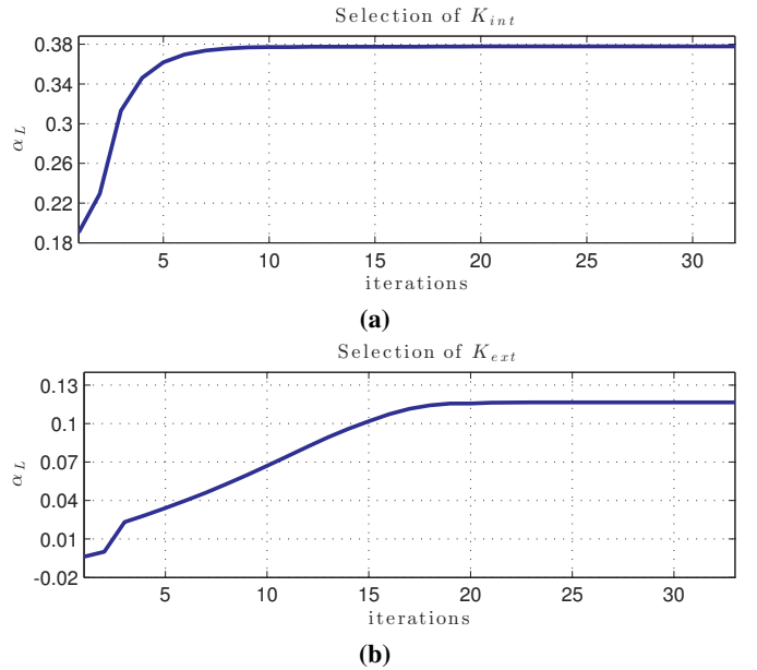
Fig. 2: Gain Selection via Algorithm 1. Evolution of \alpha_L through the iterations: (a) A_{int} and (b) A_f .
