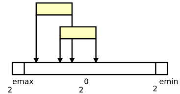
Fig. 1: Superaccumulator.
