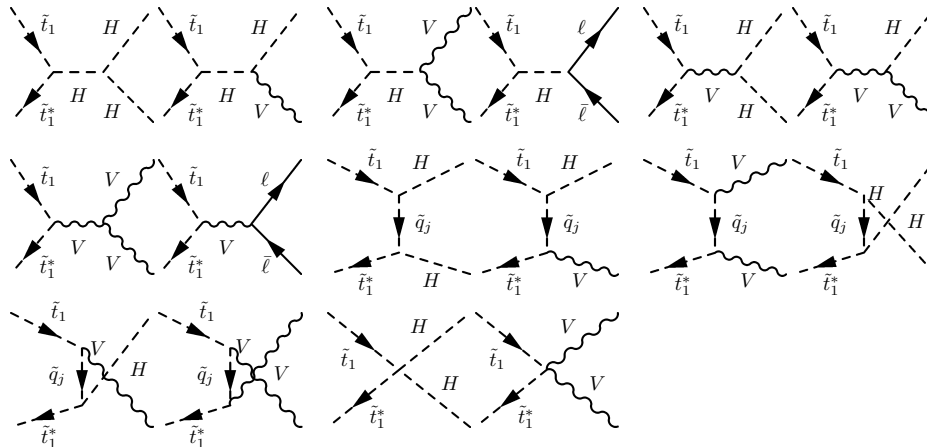
FIG. 1. Tree-level diagrams contributing to the stop annihilation into electroweak SM final states. Here, V = \gamma, Z^0, W^\pm , H = h^0, H^0, A^0, H^\pm and \ell (\bar{\ell}) can be any (anti)lepton.
