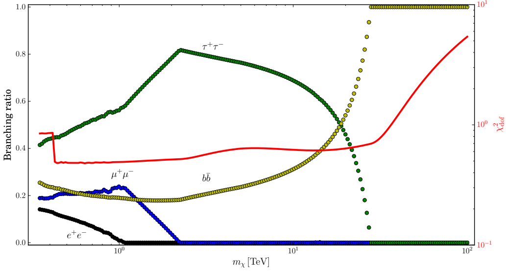
Fig. 4. Best fit for the branching fractions for each DM mass m_\chi assuming only annihilations into lepton and b\bar{b} pairs. The red line indicates on the right vertical axis the best \chi^2_{\text{dof}} value. As the DM mass exceeds the energy of the last data point, the fit improves discontinuously and the \chi^2_{\text{dof}} drops sharply, hence the kink in the red curve above 400 GeV. Between 20 and 30 TeV, the three lepton channels yield similar spectra in the range of positron energies that come into play in the fit. The branching ratio into \tau^+\tau^- should be understood as a sum over the three lepton families.
