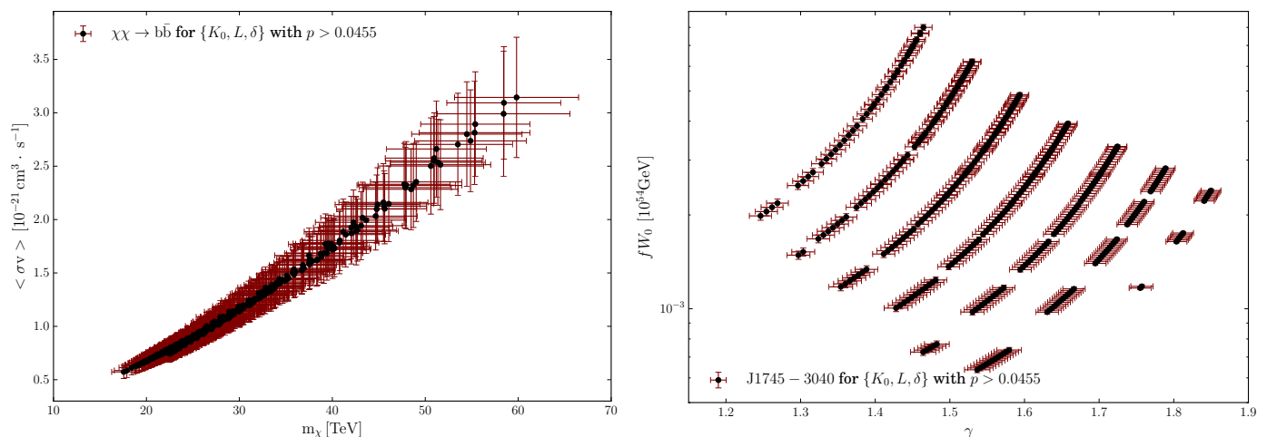
Fig. 17. Best-fit values of the surviving transport parameter sets for the DM \{m_\chi, \langle\sigma v\rangle\} (left plot) and the pulsar \{\gamma, fW0\} (right plot) parameters. The error bars represent the errors on the fit parameter resulting from the statistical uncertainty on the experimental data.
