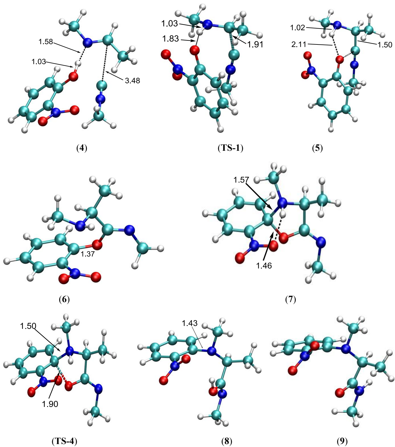
Figure 1. Optimized structures of the reaction intermediates and main transition states for the Ugi-Smiles reaction in methanol. Structures in toluene are very close. Interactive 3D structures are given for all reaction intermediates and transition states in Supporting Information.
