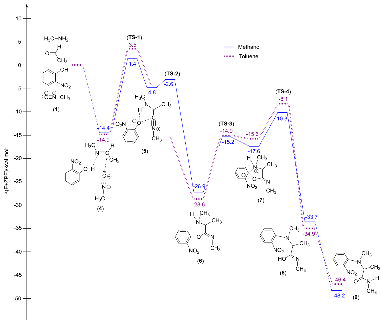
Scheme 3. Energy profile of the Ugi-Smits reaction in methanol and in toluene (at the M06-2X/6-31+G(d,p) level of theory, including ZPE corrections). The energy reference is the sum of the four reactants energies computed separately. For the sake of clarity, the water molecule released in the imine formation is not displayed in the scheme.
