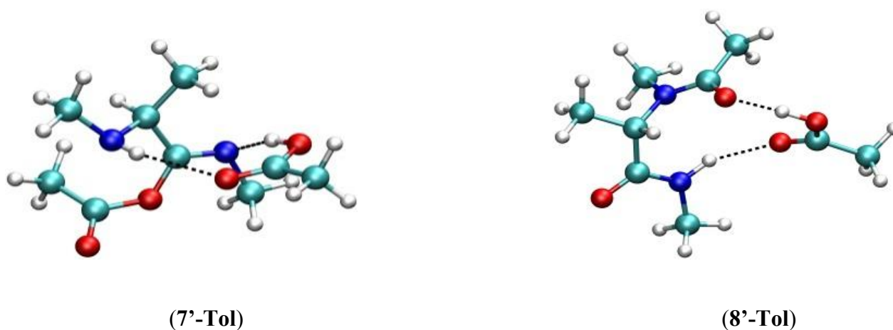
Figure 3. Optimized structures of the Mumm rearrangement with the imidate solvated by acetic acid in toluene. Structures in methanol are very close. Interactive 3D structures are given in Supporting
