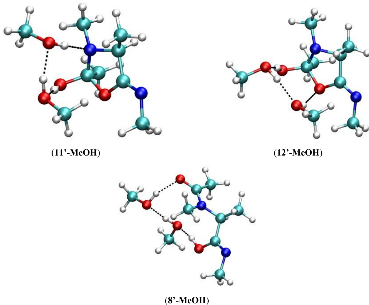
Figure 4. Optimized structures of the Mumm rearrangement with the imidate solvated by two methanol molecules. Interactive 3D structures are given in Supporting Information.
