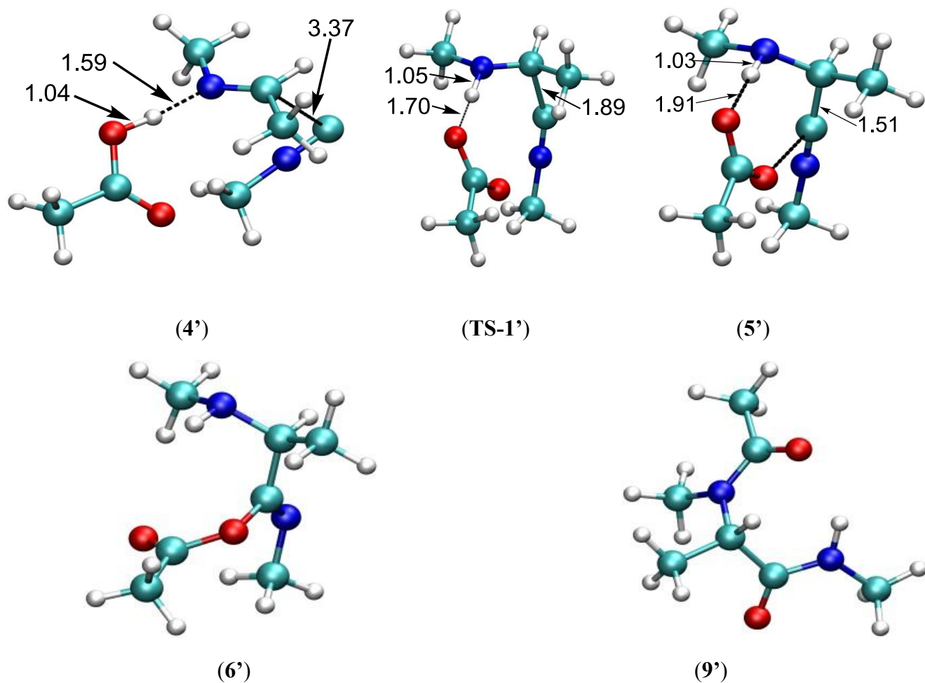
Figure 2. Optimized structures of the reaction intermediates and main transition state without microsolvation for the Ugi reaction in methanol. Structures in toluene are very close. Interactive 3D structures are given for all reaction intermediates and transition states in Supporting Information.
