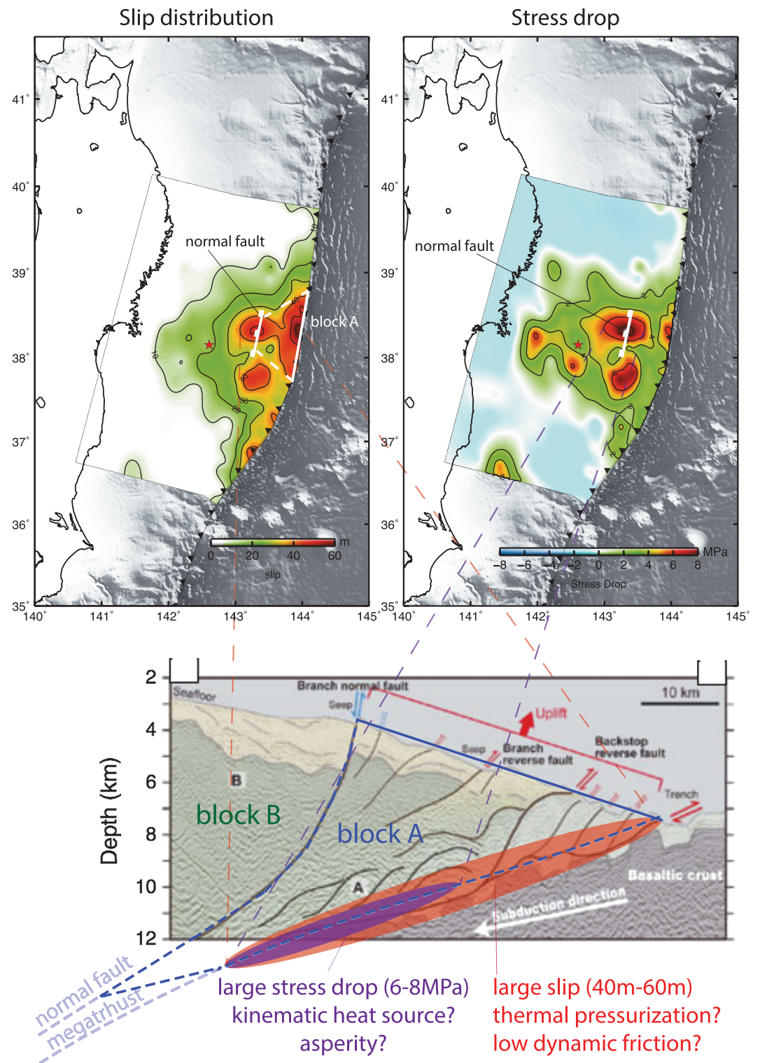
Figure 7. Illustrative sketch of the frontal wedge behavior in our proposed scenario. (top) Location of a large normal fault coseismically activated [Tsuji et al., 2011, 2013] in relation to slip (left) and stress-drop distributions (right). (bottom) Interpreted seismic profile (modified from Tsuji et al. [2011]) of the normal fault shown in top figures across the region affected by the largest slip. Blocks A (in blue) and B—separated by the large normal fault—moved by several meters in respect to each other [Tsuji et al., 2013].
