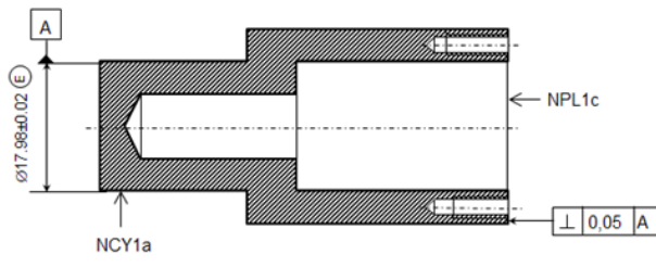
Fig. 8. Perpendicularity tolerances
