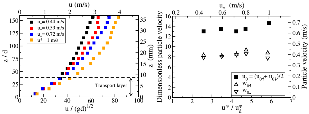
Figure 4: (a) Average particle velocity profiles obtained with natural sand of median diameter d = 230 \mu\text{m} for various wind strengths. ( u^* = 0.44, 0.59, 0.72, 1 m/s) (Ho, 2012); (b) Average horizontal slip velocity u_0 and average vertical velocity of upward and downward particles close to the bed surface ( w_{0\uparrow} and w_{0\downarrow} ) versus the friction velocity (Ho, 2012).
