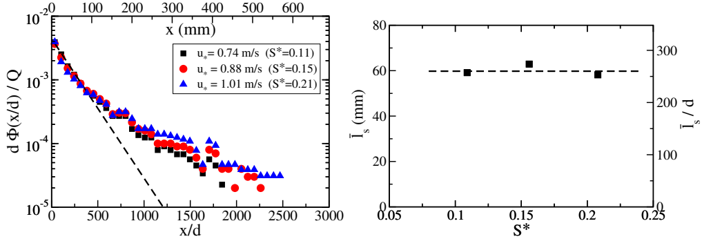
Figure 8: (a) Vertical mass flux distribution d\Phi(x)/Q for various Shields parameters (experimental data by Ho et al. (2014) with 230\mu\text{m} sand). Note that we have normalized the distribution \Phi(x) by the mass flow rate Q such that \int_0^\infty dx \Phi(x)/Q = 1 . The dash line represents the best fit to the data obtained with an exponential law. (b) Dimensionless saltation length \bar{l}_s/d versus the Shields (experimental data by Ho et al. (2014) with 230\mu\text{m} sand).
