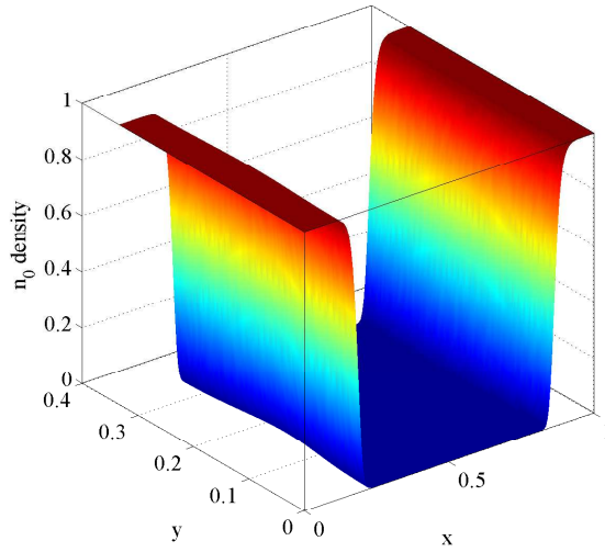
FIGURE 3. Scaled stationary charge density in a closed-state MESFET with V_D = -2 V and V_G = 1.2 V.
