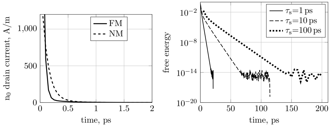
FIGURE 6. Left: Change of the electron drain current in the ferromagnetic (FM) and standard MESFET (NM), switching from open to closed state. Right: Semilogarithmic plot of the free energy versus time for various relaxation times.
