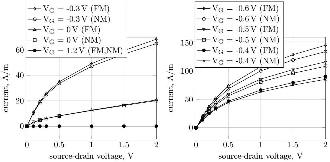
FIGURE 5. Current-voltage characteristics for the ferromagnetic (FM) and standard (NM) MESFET for various gate voltages V_G . For convenience, the source-drain voltages are given by their absolute values.
