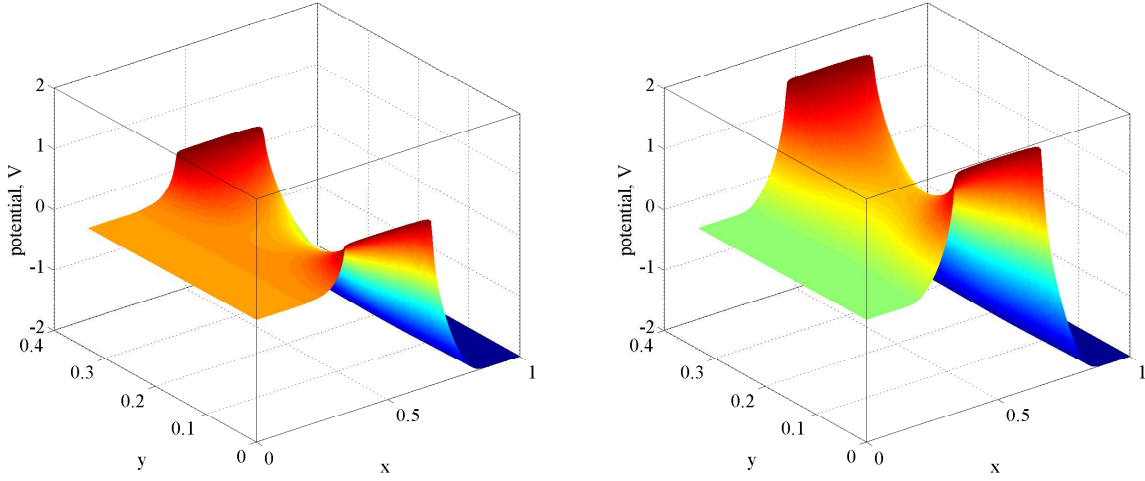
FIGURE 4. Electrostatic potential in a MESFET with V_G = 0 V (open state; left) and V_G = 1.2 V (closed state; right).
