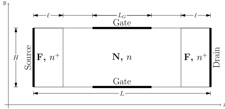
FIGURE 1. Geometry of a MESFET with ferromagnetic (F) source and drain regions and nonmagnetic (N) channel region.
